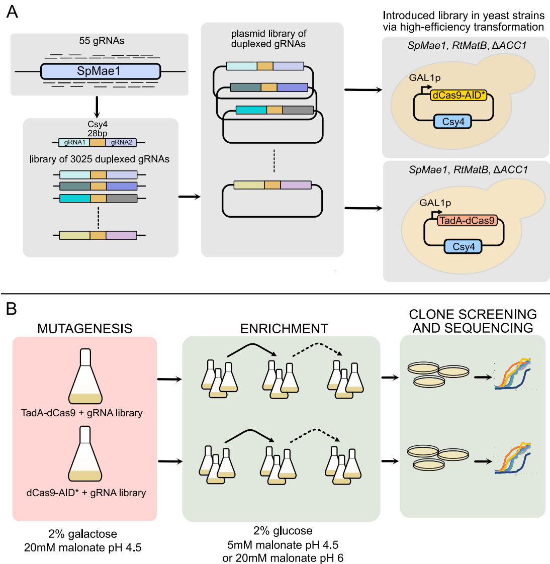
Figure 26. The SpMae1 directed evolution assay. (A) 55 gRNAs which cover SpMae1 were Csy4-dublexed in a library of 3025 variants in total which was cloned into a 2μ vector. The plasmid library was then inserted into yFlav27 ( SpMae1-RtMatB-ΔACC1 ) carrying a centromeric plasmid with either dCas9-AID* or TadA8eV106W-dCas9 under the control of GAL1p (B) The two libraries were cultivated in 2% galactose media with 20 mM malonate at pH 4.5 for mutagenesis. Next, cultures were transferred into 2% glucose media with low malonate concentration or high pH to enrich beneficial mutations. Individual clones were isolated on agar plates and screened. For spatial reasons TadA8eV106W is denoted as TadA and AID*Δ is denoted as AID*.
