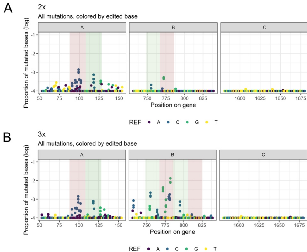
Figure 17. NGS results of the three fragments of the CAN1 gene after dCas9-AID*Δ mutagenesis when multiple gRNA arrays were used. Mutation spectra of the gRNAs 1 and 2 multiplexed (A) and all three gRNAs multiplexed (B) are shown. The x axis of each graph denotes the gene position and on the y axis the proportion of each mutation over the wild type control in logarithmic scale. The -20 bp region from the PAM site of each gRNA is shown in red and the +20 bp region from the PAM site is shown in green. Each reference base that was mutated is shown with different colour.
