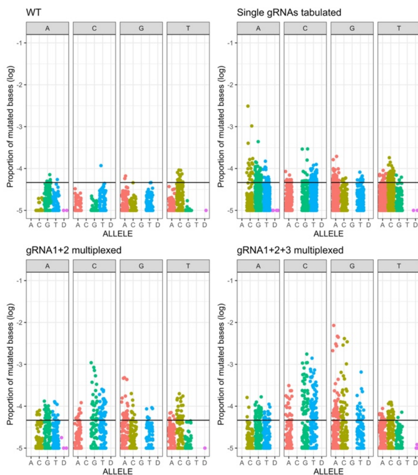
Figure 18. Base substitution frequencies of the different targeted mutagenesis experiments. The black line indicates the region in which 95% of the events are located in the WT samples. Plotted is the proportion of mutated bases for each position in the CAN1 target sequence grouped by base substitution type, with each facet representing the reference sequence base and each color representing the resulting mutated base. D denotes base deletions. Order clockwise: WT samples, tabulated data from all the single gRNA samples, all three gRNAs multiplexed, gRNAs 1 and 2 multiplexed.
