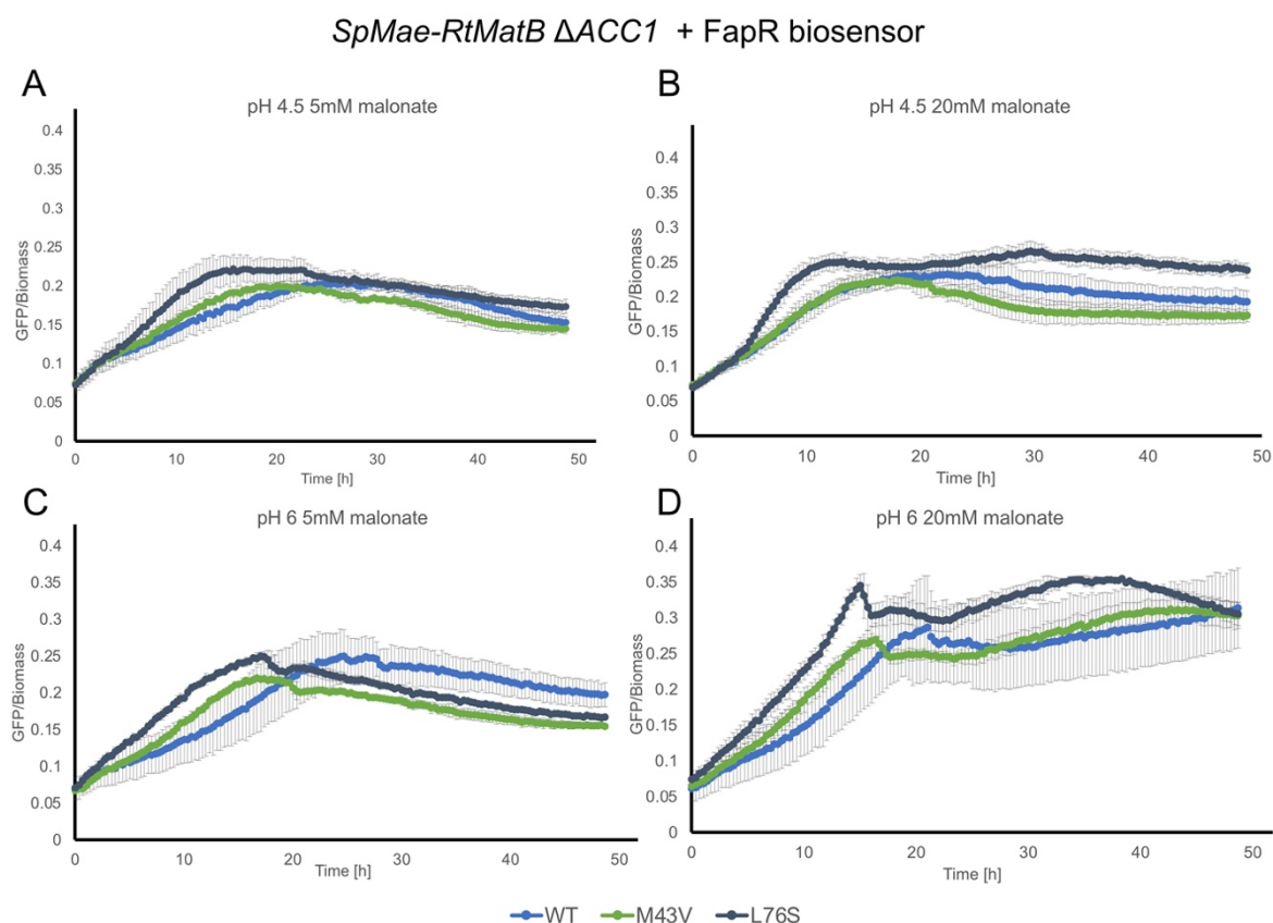
Figure 28. GFP to biomass ratio over time for the three SpMae1 - RtMatB - \Delta ACC1 + FapR biosensor strains with different SpMae1 variants. The experiment was performed in a Biolector. The y-axis represents arbitrary units. Four conditions were tested: (A) pH 4.5 and 5 mM malonate, (B) pH 4.5 and 20 mM malonate, (C) pH 6 and 5 mM malonate and (D) pH 6 and 20 mM malonate. Measurements were performed in biological triplicates and the error bars represent the standard deviation.
