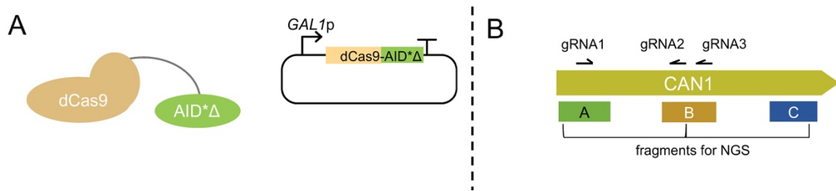
Figure 15. Overview of the experimental design for the characterization of the base editor dCas9-AID*Δ. (A): The base editor consists of dCas9 without stop codon with a C-terminus fusion of a 100 aa flexible linker and AID*Δ. The expression cassette is cloned in a centromeric plasmid under the control of GAL1p . (B): Schematic representation of the CAN1 gene and the gRNAs designed for the base editor testing, along with their direction. The 200-bp fragments (A, B, C) used for NGS are also indicated.
