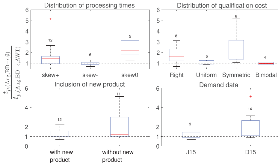
Fig. 7. Ratio of solution times for (Aug,BD- \epsilon , \phi ) versus (Aug,BD- \epsilon ,AWT) for the 23 instances in Table 3 for which the switch to AWT did occur ( \phi = 0.25 ). The number of instances in each category is specified above the corresponding box.
