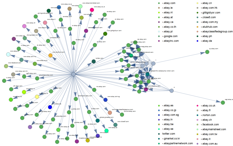
Figure A.6: Generated policies for ebay.com. The nodes with outwards pointing arrows are the five pages that we crawled. All the other nodes correspond to a possible navigation. The color indicates which part of the policy covers the navigation.
