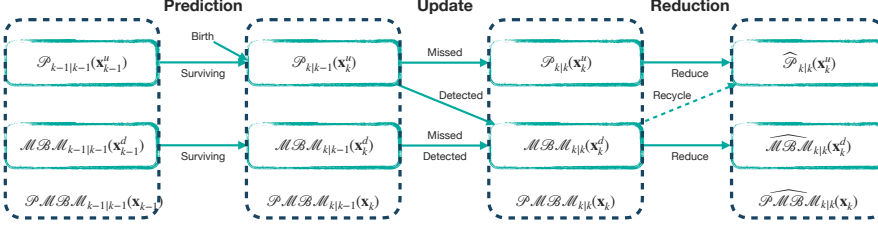
Figure 5.2: The block diagram of the PMBM filter.
