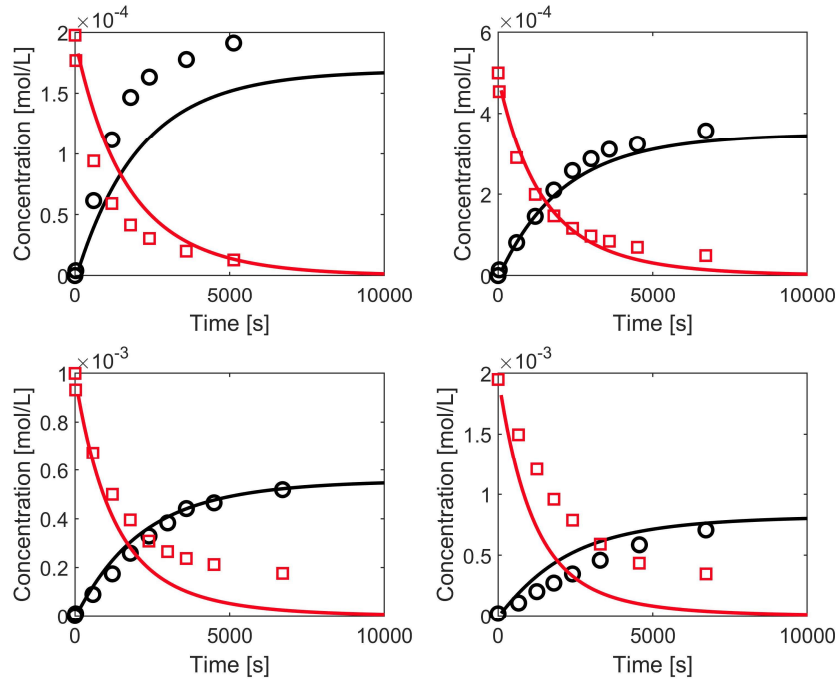
Figure 6.29. Full system fit of the Barreiro Fidalgo data [80], with stoichiometric \text{UO}_2 at t=0 with the constants ks1 , ks2 , ks3 and ks4 shown in Table 6.4.
