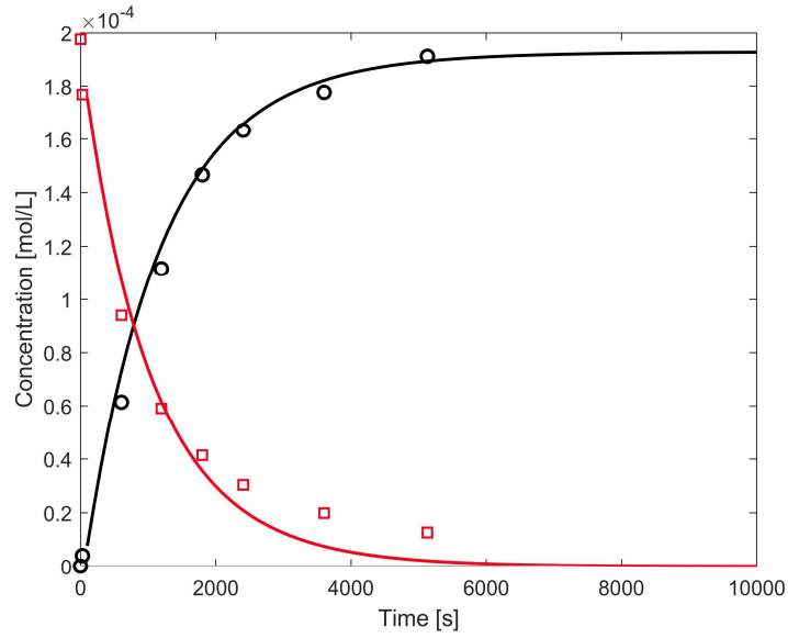
Figure 6.28. Individual data series fit of the 0.2 mM initial \text{H}_2\text{O}_2 concentration of the Barreiro Fidalgo data, with stoichiometric \text{UO}_2 at t=0 with the constants ks1 , ks2 , ks3 and ks4 shown in Table 6.4.
