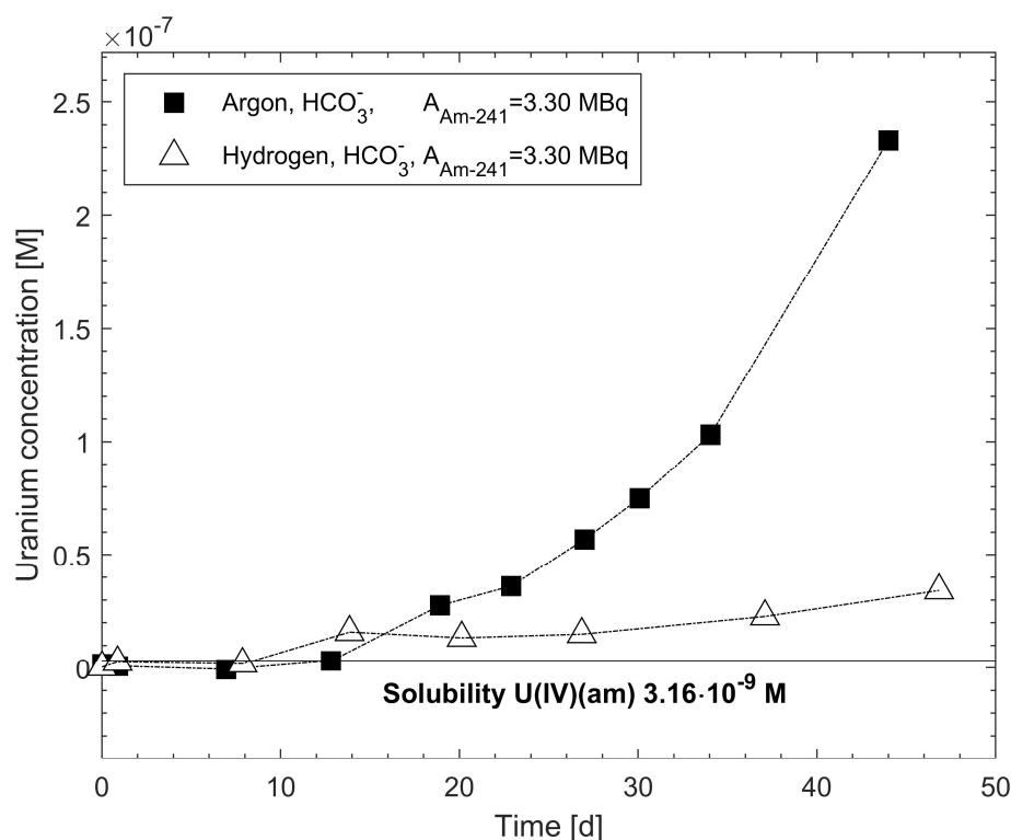
Figure 6.2. Dissolved uranium concentrations in 10 mM \text{NaHCO}_3 solution in contact with the \text{UO}_2 pellet next to the 3.30 MBq \text{Am-241} source under Ar and \text{H}_2 atmospheres. The \text{U(IV)(am)} solubility is taken from the work of Neck and Kim [47].
