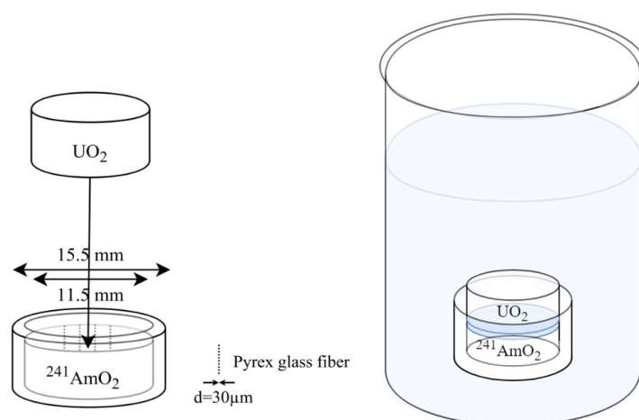
Figure 5.1. \text{UO}_2 pellet separated by 30\text{ }\mu\text{m} from the \text{Am-241} source by placing Pyrex glass fibres in-between.
