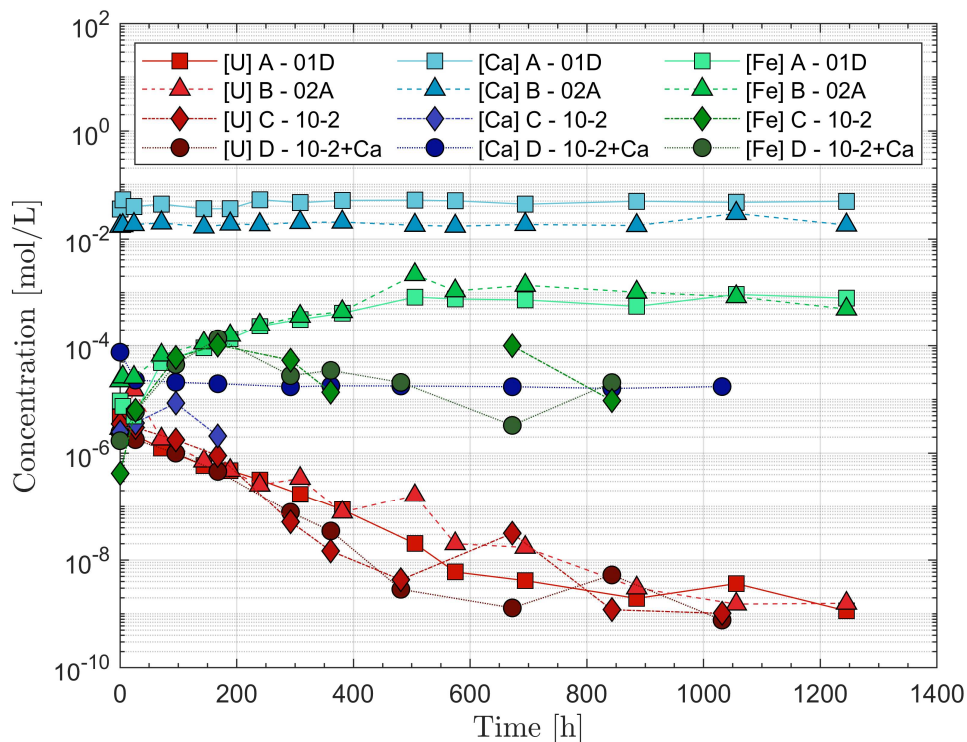
Figure 6.13. 3000 ppm \text{CO}_2 in Ar atmosphere batch experiment with samples A-D using the \text{FeSO}_4 \text{O}_2 -trap.
