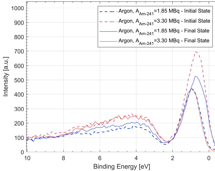
Figure 6.11. Valence band region showing the O2p and U5f peaks of the \text{UO}_2 pellets exposed to the 1.85 and 3.30 MBq \text{Am-241} sources under Ar atmosphere.
