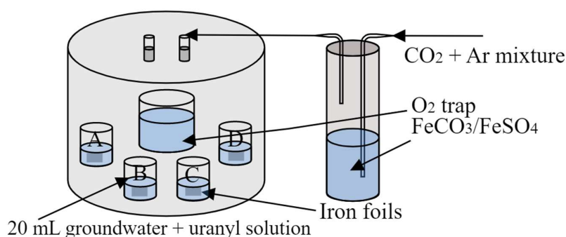
Figure 5.2. Experimental setup for the iron foil experiments, with reaction vessel and gas washing bottle containing \text{O}_2 -traps and groundwater + uranyl solutions. The setup was kept in the inert glovebox atmosphere throughout the experiment.
