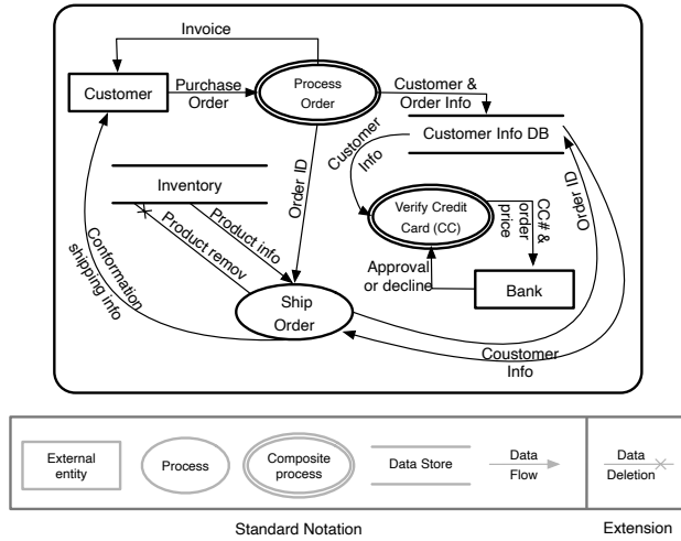
Figure 1.2: Example of a Data Flow Diagram (DFD). The ‘data deletion’ element is an extension to the standard DFD notation (Business-oriented DFD (B-DFD)).
