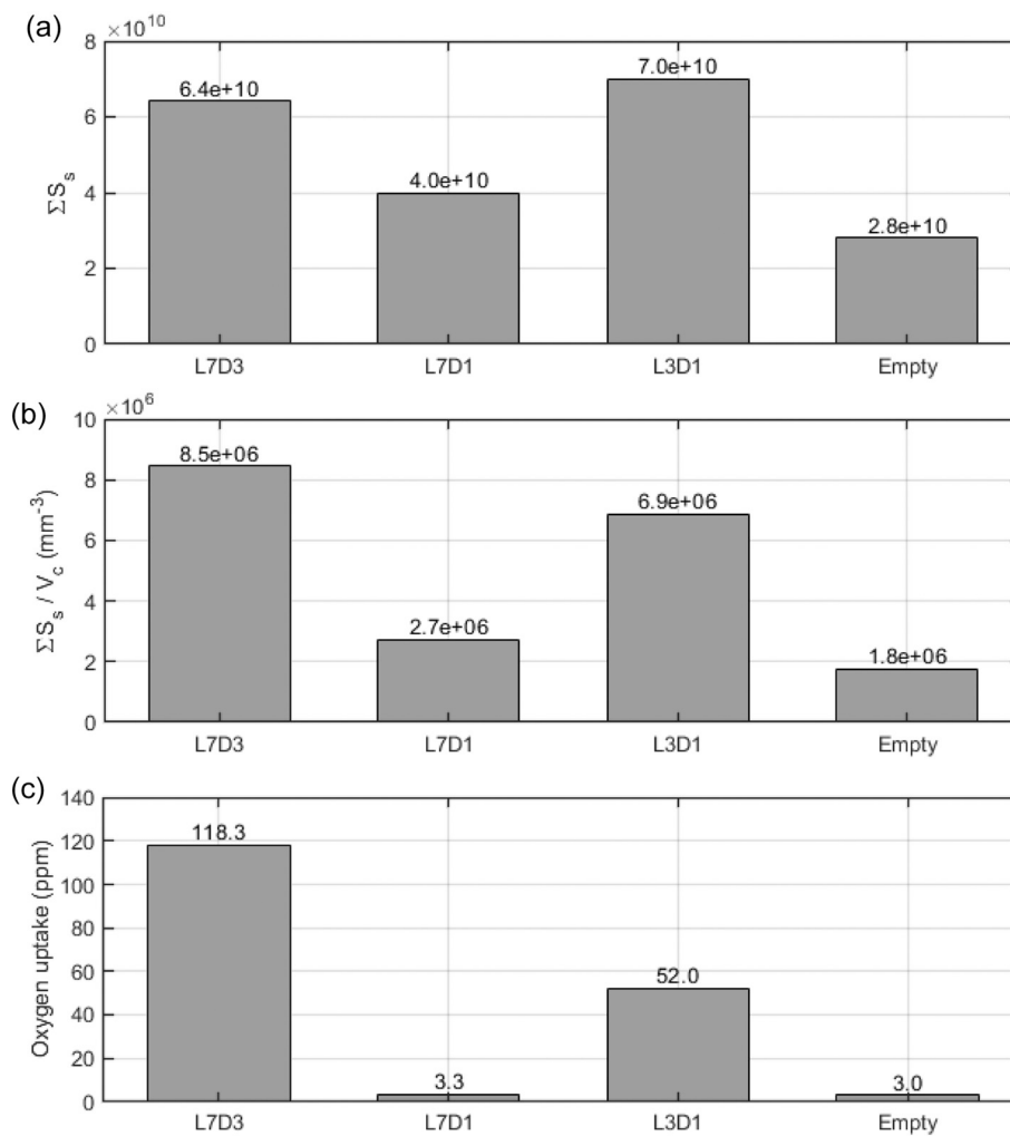
Fig. 12. Comparisons of (a) total GVs in the spatter region \Sigma S_s , (b) GVs per unit volume of cavity in the container \Sigma S_s / V_c , (c) oxygen uptake compared to virgin state in the four containers.
