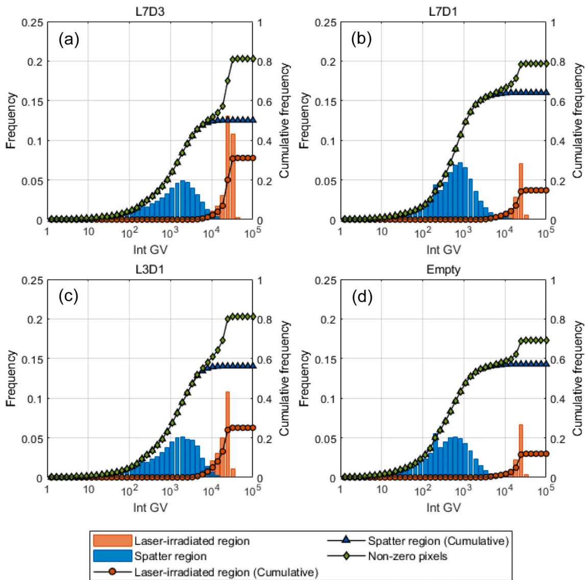
Fig. 3. Histograms of GVs in the OT images of all layers identified as the laser-irradiated regions and the spatter regions for the (a) L7D3, (b) L7D1 (c) L3D1 and (d) empty containers. The frequency values are normalized by the total count of pixels in the bounding boxes of the container samples. On the right axes, the cumulative frequencies for both regions are plotted. The cumulative frequency of non-zero pixels combines both regions. The cumulative frequency plots of non-zero pixels do not reach unity since there are zero GV pixels present in the evaluated volumes.
