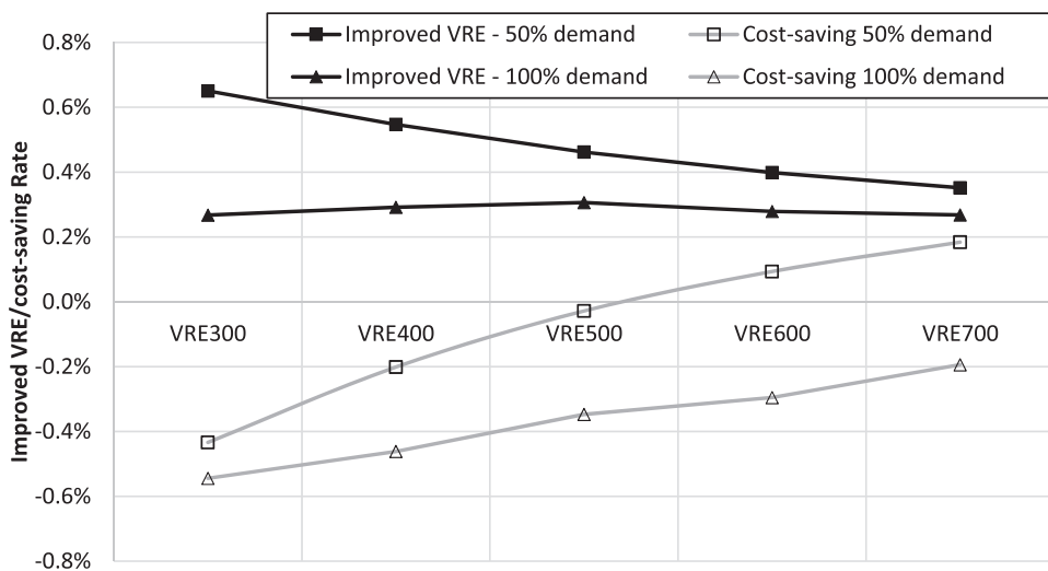
Fig. 18. Improved VRE integration rate and cost-saving rate for the MTDH systems with back-pressure plant under different conditions.
