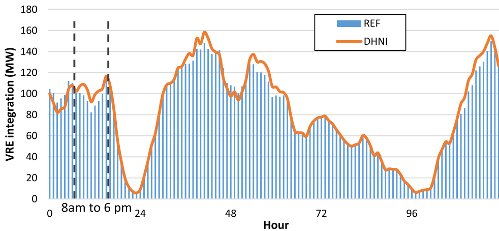
Fig. 10. Hourly VRE integrations of the REF and DHNI systems for five typical days from Jan 1st to Jan 5th.
