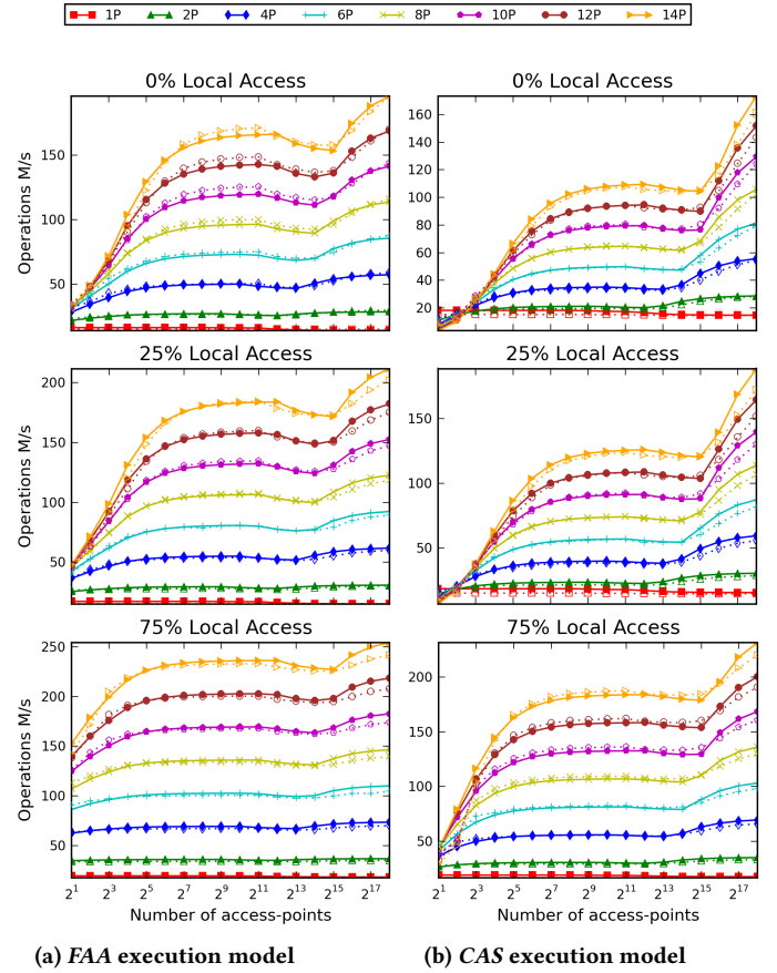
Figure 2: General model validation, Xeon CPU. Solid lines present the model throughput prediction, dashed lines present the actual measured throughput, P stands for thread(s).
