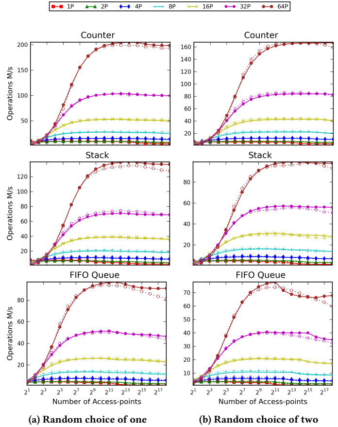
Figure 5: Data structures model validation, XeonPhi CPU. Solid lines present the model prediction, whereas the dashed lines present the actual measured throughput. P stands for thread(s).
