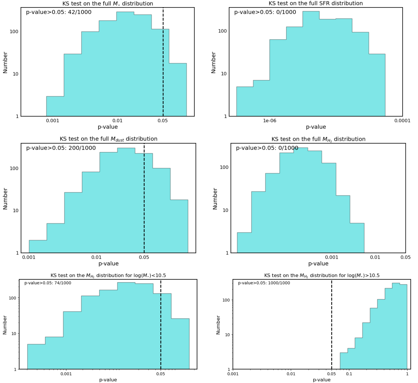
Fig. A.1. KS tests: results. Upper panels: Histograms of the p-values of the KS test performed on the simulated M_{\star} (left panel) and SFR (right panel) distributions of AGN and the control sample of SFGs. On the y axis, the logarithm of the number of entries is divided into ten equally log-spaced bins, and the p-values resulting from the 1000 KS tests are reported on the x axis. The threshold above which we cannot reject the null hypothesis that the samples are drawn from the same distribution is represented by a vertical, dashed black line at p = 0.05 . Central panels: Same as the upper row, but with M_{\text{dust}} (left panel) and M_{\text{H}_2} (right panel) distributions. Bottom panels: Results of the KS tests on the M_{\text{H}_2} distribution in the \log(M_{\star}) < 10.5 M_{\odot} (left panel) and \log(M_{\star}) > 10.5 M_{\odot} (right panel) regimes.
