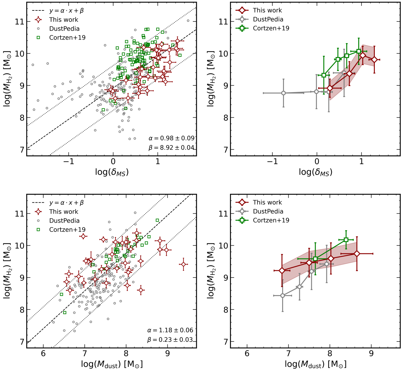
Fig. 6. Comparison of the molecular gas properties, part II. Left panels: molecular gas mass ( M_{\text{H}_2} ) versus the offset from the MS (derived assuming the relation by Sargent et al. 2014; top panel ) and host-galaxy dust mass ( M_{\text{dust}} ; bottom panel ). Seyfert 2 galaxies are shown with red diamonds, and the control sample is represented by gray circles (DustPedia) and green squares (Co19). Bottom panel: we show the M_{\text{H}_2} - M_{\text{dust}} diagram, where the M_{\text{H}_2} of the 33 5MUSES SFGs were derived from the CO luminosity (Co19), assuming \alpha_{\text{CO}} = 4.3 M_{\odot} \text{ pc}^{-2} (\text{K km s}^{-1})^{-1} . We do not represent the entire sample of 5MUSES SFGs since their M_{\text{H}_2} are derived from the M_{\text{dust}} assuming a dust-to-gas ratio (GDR). For purely illustrative purposes, the best-fit trend (dashed black line) for the control sample of inactive galaxies is shown, and the two dotted black lines are the same trend shifted by a factor of 0.5 dex in either direction. The best-fit slope ( \alpha ) and normalization ( \beta ) are reported in each panel. Right column: same scaling relations presented on the left, but with binned values (using the same method as in Fig. 5). The red-shaded regions are as described in Fig. 5.
