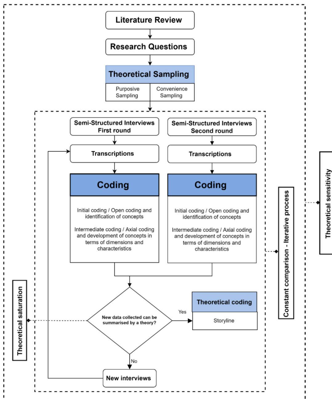
Figure 1. Research framework.
