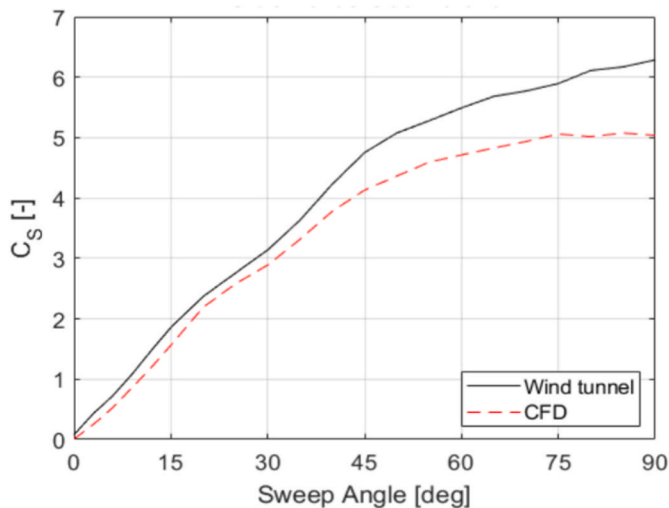
Fig. 10. Comparison between wind tunnel and CFD results for the aerodynamic side force coefficient obtained for simplified truck model.
