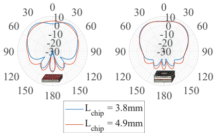
Fig. 10. Directivity for single-element antenna element with 2 rows of pins with (right) and without (left) the top PCB.
