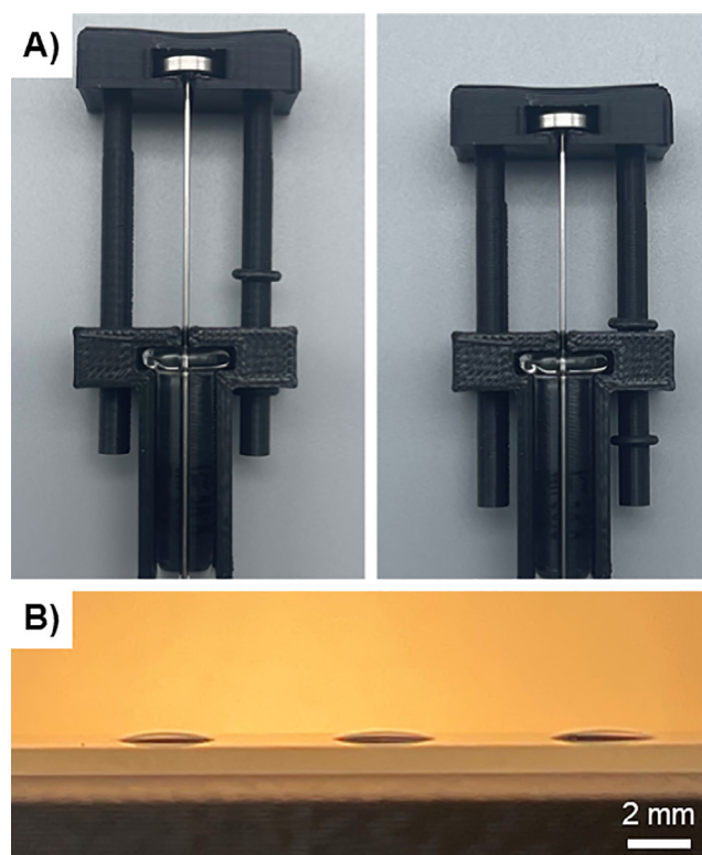
Fig. 11. A) Photos showing the plunger before dispensing (left) and after dispensing the target volume (right) (3 \mu\text{L} ). B) 3 \mu\text{L} of DI water dispensed three-times on glass slide.
