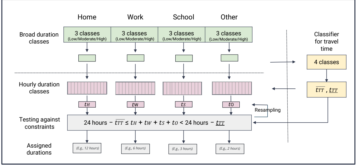
Figure 4.2: The flow chart of activity duration assignment methodology in SySMo.
