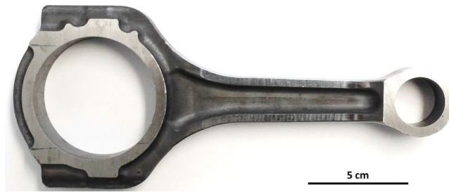
Figure 1. Photo of the connecting rod.
