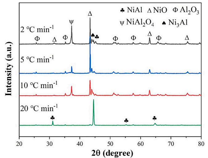
Fig. 15. XRD patterns of the oxidation products of porous NiAl at 900 °C for 120 h.
