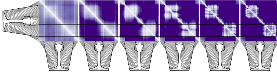
Figure 10: Transfer function from the velocity at each individual surface node (y-axis) to the sound pressure at each surface nodes (x-axis), displayed as the relative difference to the largest contribution, in dB. Left to right: 25 Hz, 500 Hz, 1000 Hz, 2000 Hz, 4000 Hz, and 7500 Hz.
