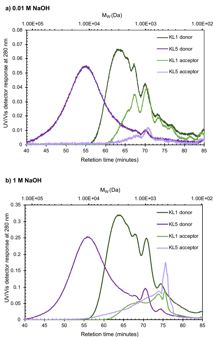
Figure 9 Comparison between SEC chromatograms of donor and acceptor samples for KL1 and KL5 in the a) 0.01 M NaOH solution and b) 1 M NaOH solution. The secondary x-axis above the graphs shows the M_w values calculated based on a calibration curve from PEG standards.
