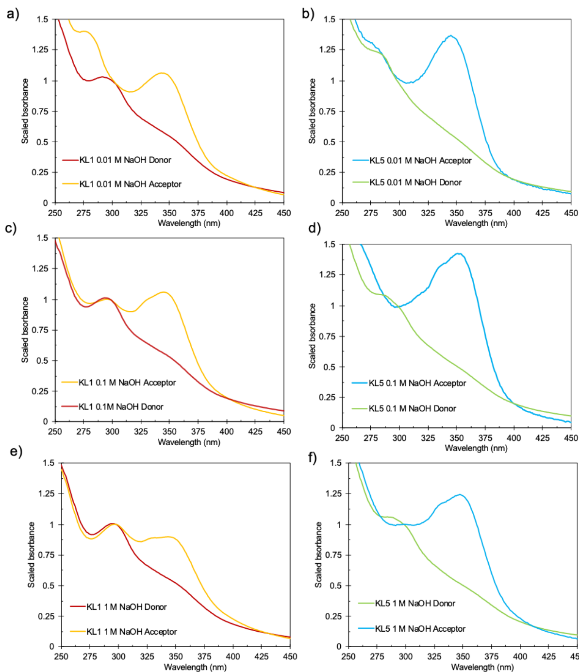
Figure 10 Scaled UV/Vis absorbance spectra of the donor (at the start) and acceptor (after 168 h) samples of a) KL1 in 0.01 M NaOH, b) KL5 in 0.01 M NaOH, c) KL1 in 0.1 M NaOH, d) KL5 in 0.1 M NaOH, e) KL1 in 1 M NaOH, and f) KL5 in 1 M NaOH.
