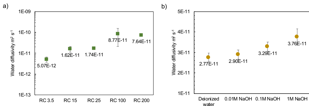
Figure 2 Water diffusivity through different membranes, measured as the diffusion of tritium oxide a) through pretreated RC membranes with various pore sizes (RC3.5, RC15, and RC25, representing MWCOs of 3.5, 15, and 25, respectively and RC100 and RC200 representing membranes with nominal pore sizes of 100 nm and 200 nm) in neutral conditions and b) through the 50 kDa MWCO membrane (RC50) in different alkalinities.
