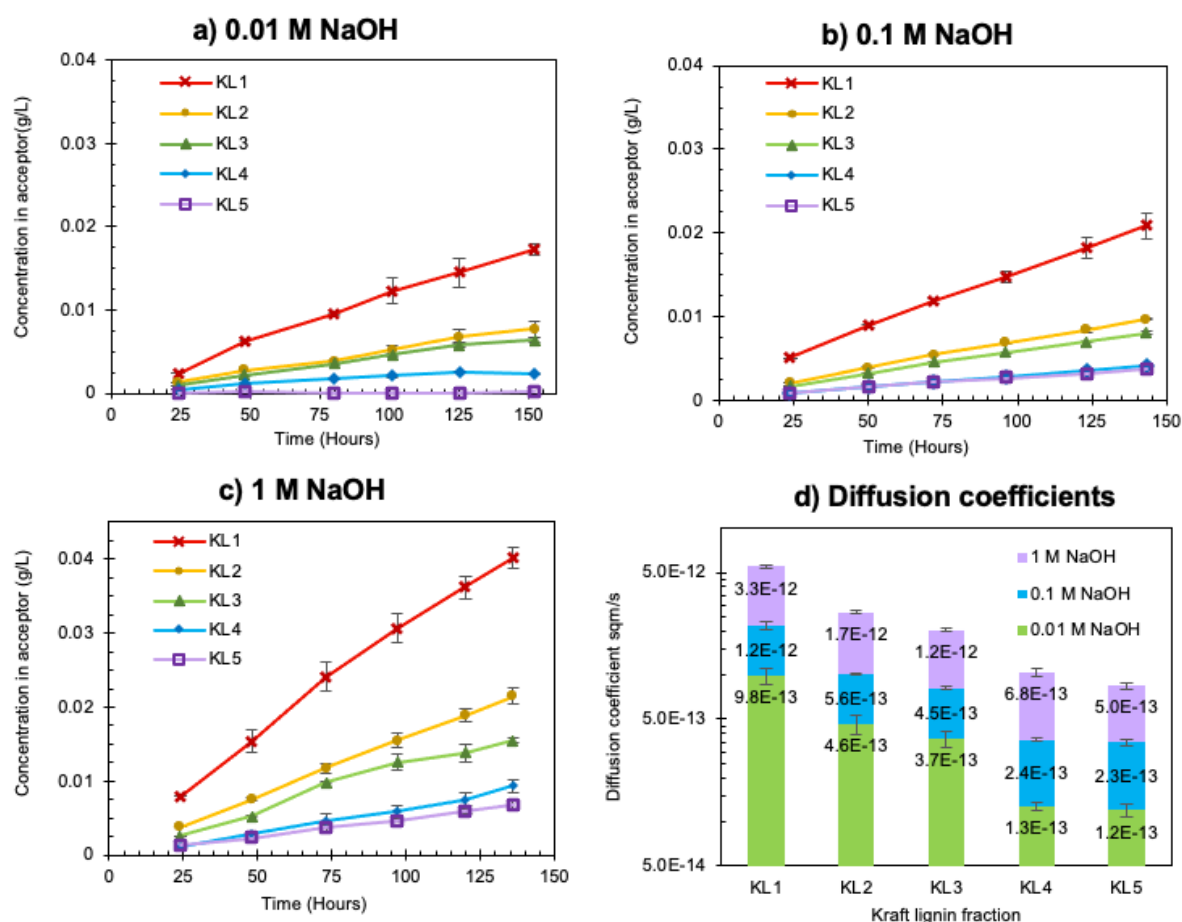
Figure 7 Concentration of lignin in the acceptor chamber versus time in the a) 0.01 M NaOH solution, b) 0.1 M NaOH solution, and c) 1 M NaOH solution, together with d) a summary of the fractionated diffusion coefficients of lignin measured from the diffusion cells. The concentrations were determined by UV/Vis absorbance according to a calibration curve for kraft softwood lignin in alkaline solutions.
