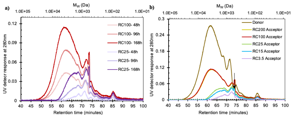
Figure 5 SEC chromatogram curves showing the UV detector response at 280 nm versus retention time for a) the acceptor samples that passed through RC100 and RC25 membranes at three diffusion times and b) the donor sample and acceptor samples that passed through various membranes after 168 h. The arrow refers to the peak at 73 min. The secondary x-axis above the graphs shows the M_w values calculated based on a calibration curve from PEG standards.
