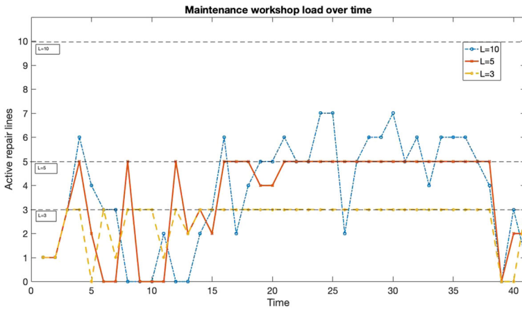
Fig. 6 Maintenance workshop load over time for (I, J_i, K, T, b^i) = (5, 15, 10, 40, 1) and L \in \{10, 5, 3\} . Points on the Pareto front for objectives (10) and (8): availability = 5; maintenance cost \in \{5542, 5546, 5631\} ; no constraints on the stock levels at the end of the planning horizon
