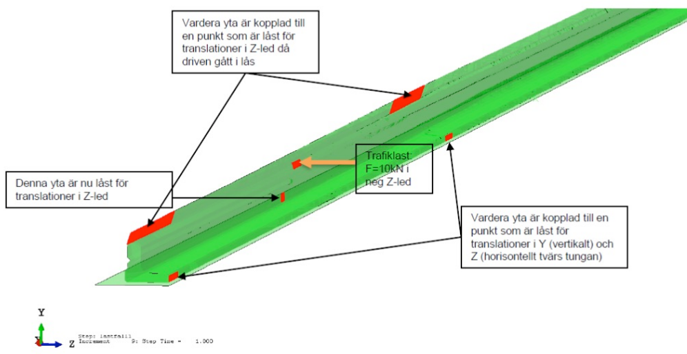
Figure 30 Description of how boundary conditions are modelled.
