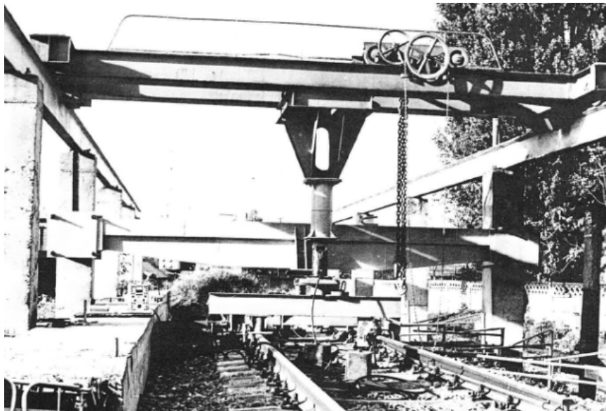
Figure 17 General view of the test rig used. From [5].
