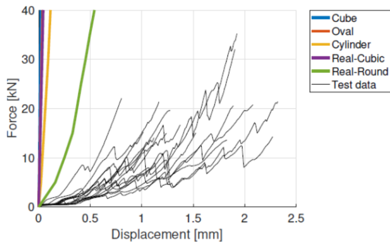
Figure 21 Displacement predicted by FE analyses and evaluated from test data. From [1].
