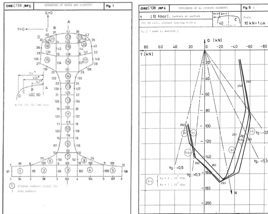
Figure 16 Examples on FE-mesh and isobar for UIC60 and 60 cm sleeper spacing. From [5].
