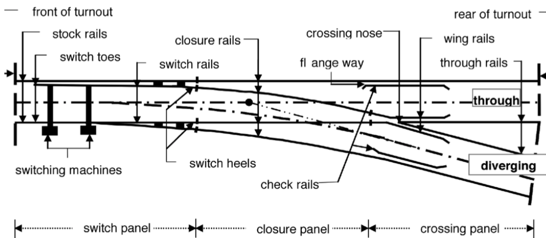
Figure 1 Switch components nomenclature. From [1].
