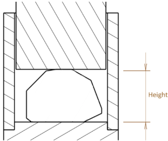
Figure 20 Cross section of the hydraulic press test set up. From [1].
