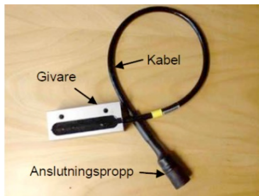
Figure 3 Contact for eTKK2. (Givare = sensor, Kabel = cable and Anslutningspropp = Connection plug). From [2].
