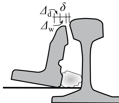
Figure 27 Cross-sectional deformation due to loads from drives and a wheel.
