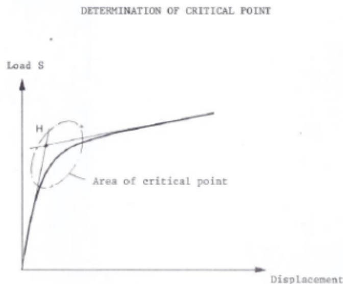
Figure 14 Load displacement curve to find the area of critical point H regarding track shift. From [5].
