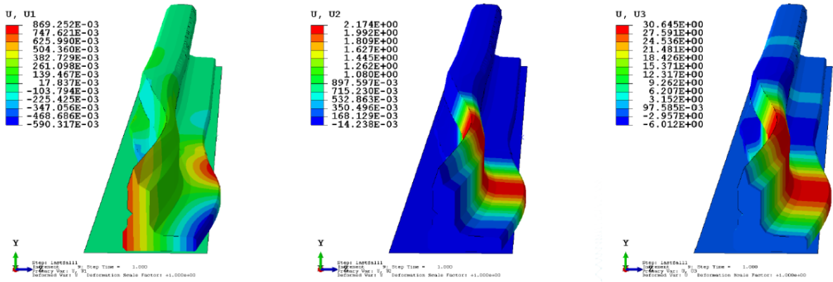
Figure 31 Deformation of a locked switch rail due to a prescribed 30 mm horizontal deformation of the rail foot.
