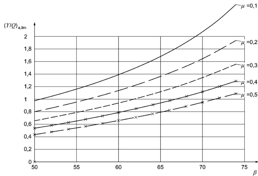
Figure 9 Limit values for (Y/Q) for variation in the flange angle \beta and the friction coefficient \mu . From [2].
