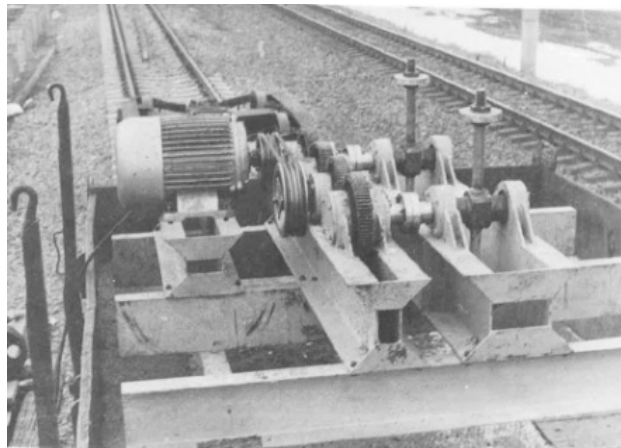
Figure 15 View of the vibrator used in tests. From [5].
