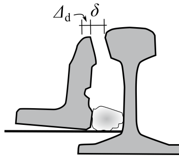
Figure 26 Cross-sectional deformation due to loads from the drives.
