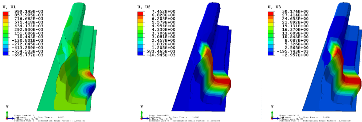
Figure 32 Deformation of a locked switch rail with a 30 mm rail foot deformation due to an applied horizontal wheel load acting on the switch rail head.
