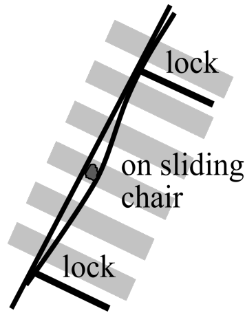
Figure 25 Sketch of the locked drives and the trapped ballast stone.
