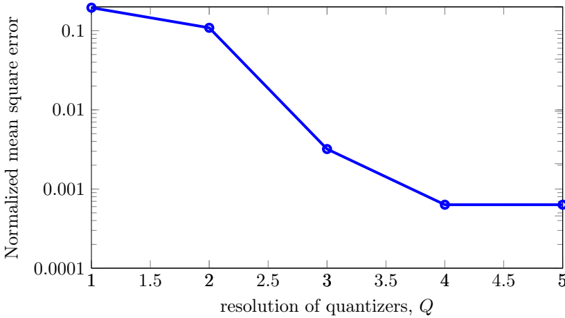
Figure 3.2: Diagonal approximation accuracy for different quantization resolution. The number of antennas
