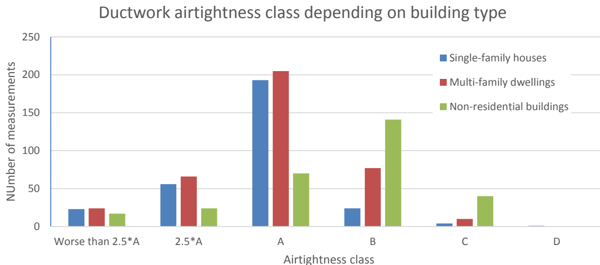
Figure 3: Specific ductwork airtightness measured class depending on the building type
