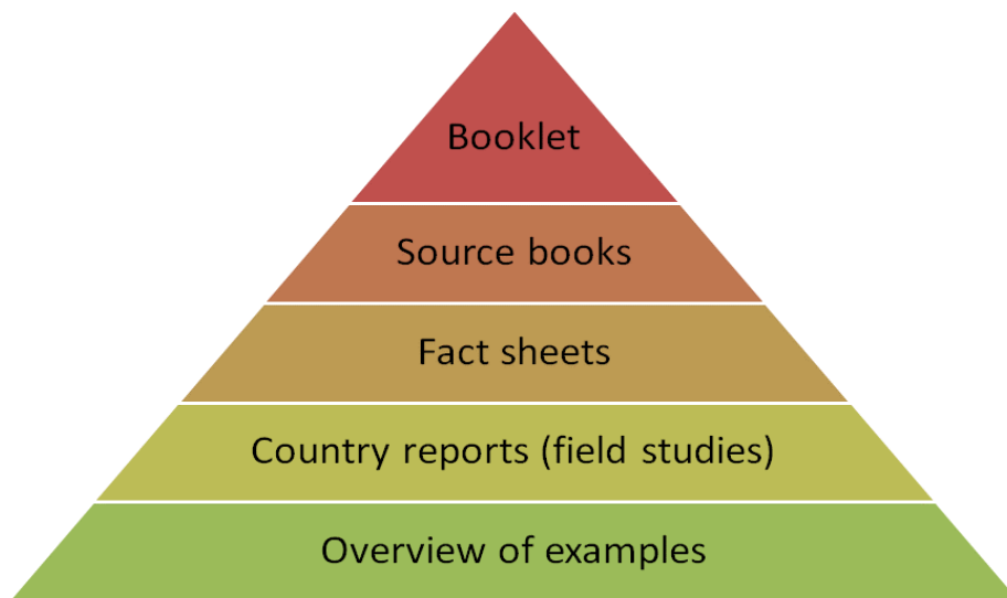
Figure 1: QUALICHeCK deliverables
