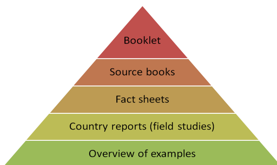
Figure 5: QUALICHeCK deliverables
