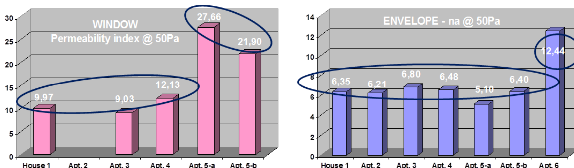
Figure 21 Air permeability index of windows (left) and envelope air change rate (right)
