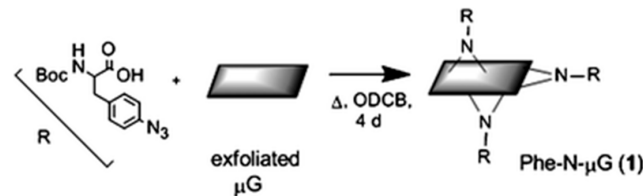
Scheme 9. Nitrene addition to exfoliated micro-crystalline graphite in refluxing o -dichlorobenzene (ODCB). Reproduced with permission from [25], copyright 2010 The Royal Society of Chemistry.
