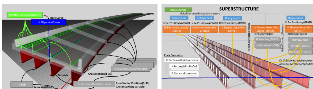
Figur 6: IFC4.3 (BuildingSmart).
