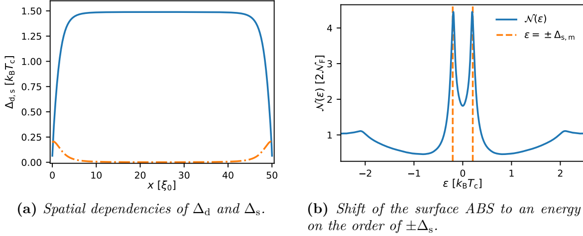
Figure 4.7: Enhancement of a sub-dominant order parameter \Delta_s close to a partially reflective pair-breaking surface where the dominant d-wave pairing is suppressed. The interfaces is characterized by D_0 = 0.5 and \beta = 1 , see Eq. (2.75), and a misalignment angle of \alpha = \pi/4 . The temperature T = 0.1T_{c,d} \approx 0.5T_{c,s} and we have \Gamma = 0.01\pi k_B T_c in the Born limit.
