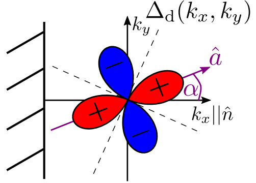
Figure 4.5: The angle \alpha measures the misalignment of the crystal \hat{a} axis and the normal of a crystal surface.
