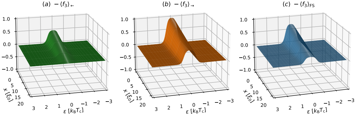
Figure 5.4: The charge mode for (a) left-movers, (b) right-movers, and (c) FS-averaged. Note that we show -\langle f_3 \rangle_{\rightarrow/\leftarrow/\text{FS}} is shown and the x and \varepsilon axes are flipped compared to Fig. 5.3.
