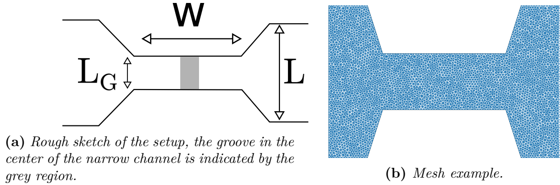
Figure 5.26: Grooved Dayem bridge: Sketch and mesh.
