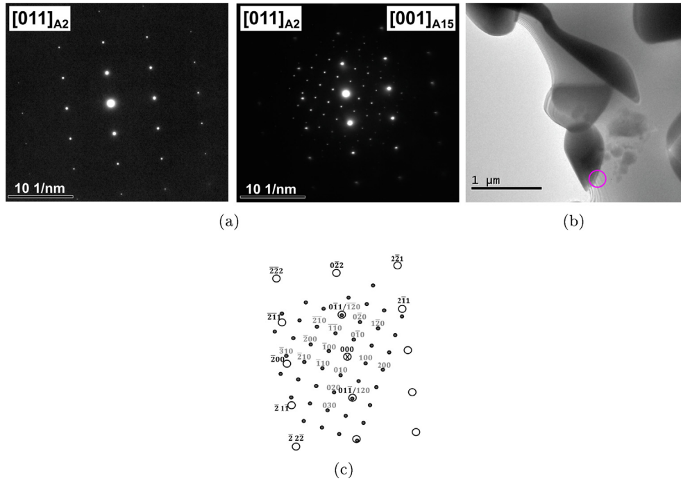
Fig. 6. SADPs of the Cr ss matrix (A2 structure) and the Cr ss /A15 interface of the Cr 91 Si 9 alloy after 100 h at 1200°C annealing are shown in (a). In (b) the corresponding microstructure with the interface from which the SADP was taken (marked) and in (c) an indexed schematic of (a) are shown.
