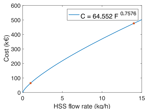
Fig. 17. Cost function reclaimer, material: welded SS316. The sizing parameter (F) for the reclaimer is the HSS flow rate (kg/h).
