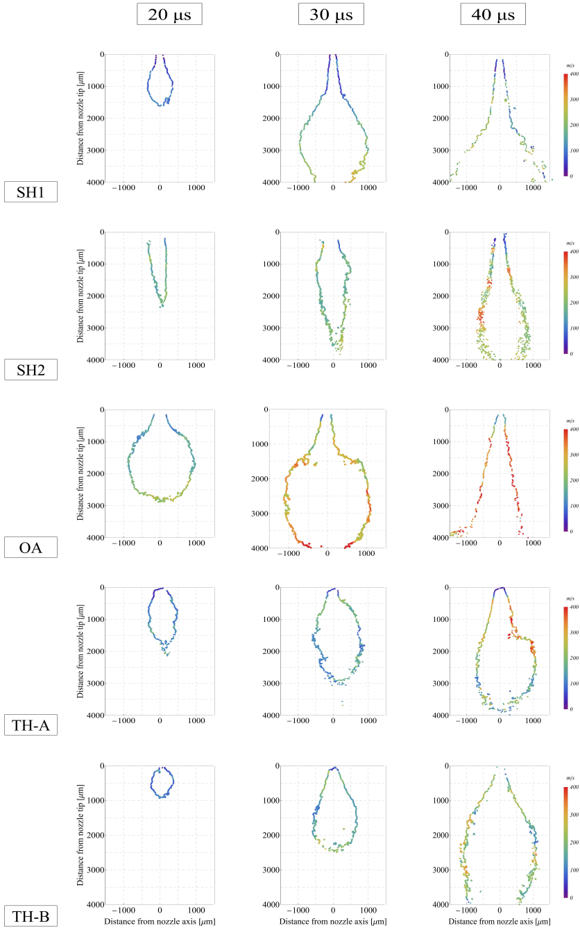
Figure 4.2: Mean velocity magnitude for near-field sprays generated by five different orifices at 1600 bar
