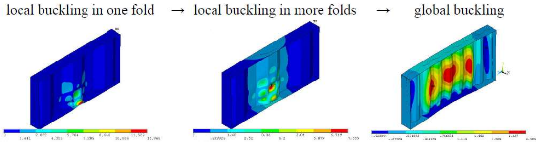
Figure 3.3 Different failure modes (Kövesdi, 2010)
