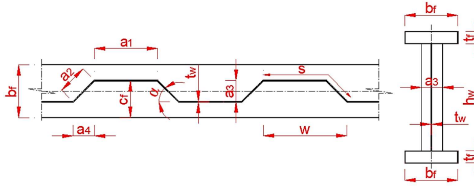
Figure 1.1 Notations used for trapezoidal corrugated web
