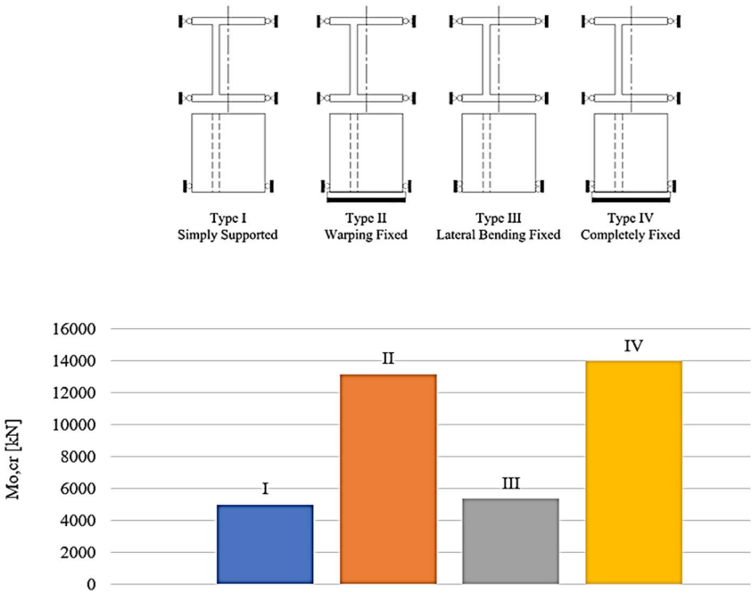
Figure 1.33 Elastic critical buckling moment for different boundary conditions, the calculation according to (Nguyen, Han et al. 2011)
