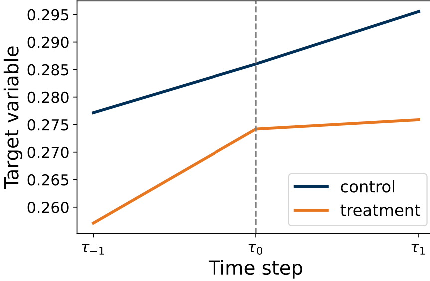
Figure 8.7: Target variable y measured before the treatment ( \tau_{-1} ), when the treatment is applied ( \tau ), and after the treatment ( \tau_1 ), for the control and the treatment groups, y is min-max scaled.
