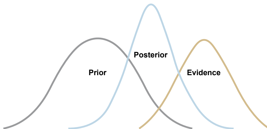
Figure 2.4: An illustration of Bayesian inference of prior, evidence, and posterior distributions.
