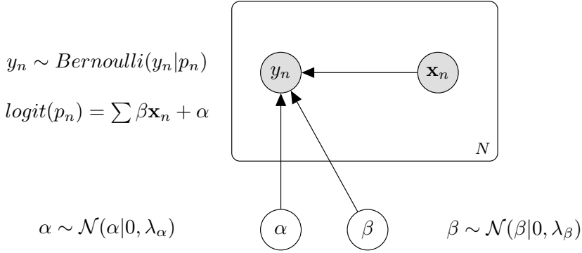
Figure 7.1: Probably graphical model of a Bayesian logistic regression, with observed input features ( \mathbf{x}_n ), treatment indicator ( y_n ), and latent variables as regression model coefficients ( \alpha, \beta ).
