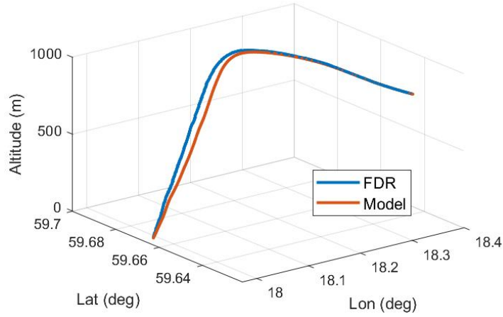
Figure 2.5: 3D flight path comparison.
