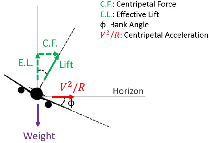
Figure 2.1: Free body diagram of an aircraft in banked turn.
