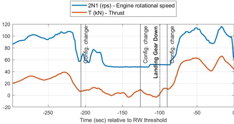
Figure 2.3: Thrust estimation compared to engine rotational speed data.
