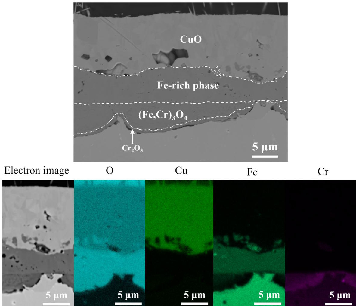
Figure 25: BIB-milled cross-section of a TS Cu-coated sample of 441 that was exposed at 650\ ^\circ\text{C} in humid air for 1,000 h, together with the corresponding EDS analysis.
