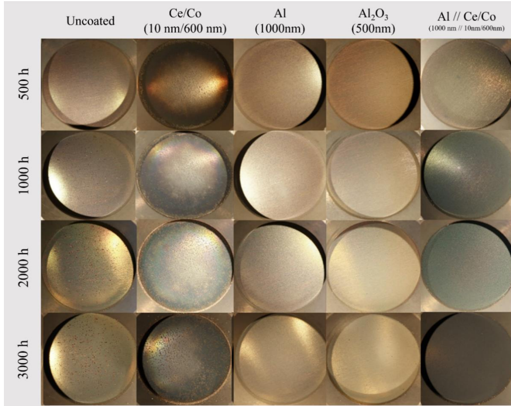
Figure 28: Photographs of the air-facing sides of AISI 441 coupons taken during discontinuous dual-atmosphere exposure ( \text{Ar-5\% H}_2 + 3\% \text{H}_2\text{O} // \text{Air} + 3\% \text{H}_2\text{O} ) at 600^\circ\text{C} .
