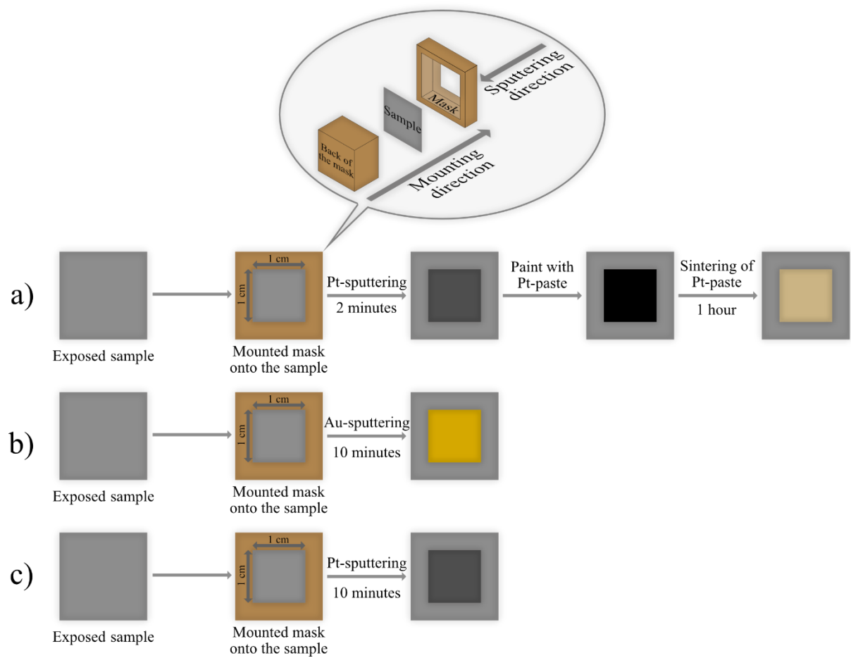
Figure 18: Schematic of the electrode preparation process [122].
