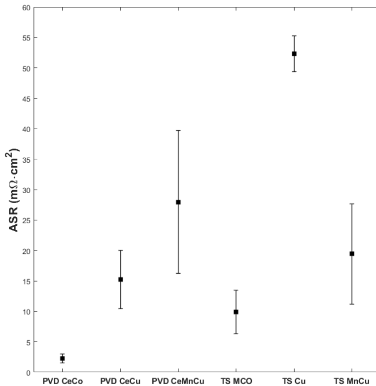
Figure 39: ASR measurements in air for samples exposed at 650°C for 1,000 h in air + 3% H 2 O. Error bars indicate standard deviation.
