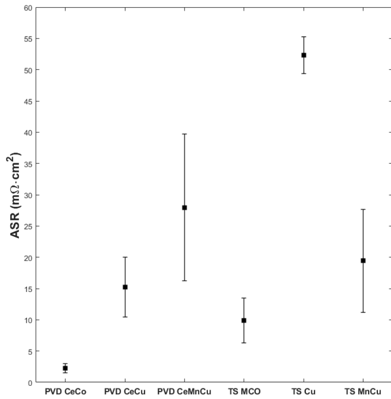
Figure 27: ASR measurements in air of samples that were exposed at 650 °C for 1,000 h in air + 3% \text{H}_2\text{O} . Error bars indicate standard deviation.
