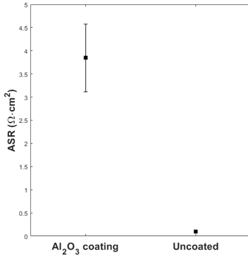
Figure 48: ASR measurements of PVD Al 2 O 3 -coated sample and uncoated sample, exposed to Ar – 5% H 2 – 3% H 2 O with a flow rate of 120 smL·min -1 for 668 h at 600°C. The error bars represent the maximum and minimum values measured.
