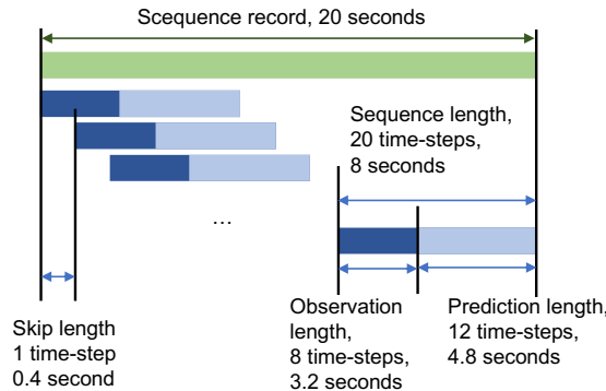
Figure 1.14: How the training and evaluation sequences are cut.
