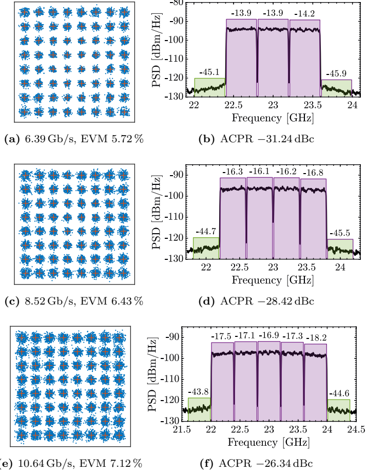
Figure 7.6: Constellation diagram and output spectrum for (a)-(b) three aggregated 400 MHz OFDM channels, (c)-(d) four aggregated 400 MHz channels, and (e)-(f) five aggregated 400 MHz channels, respectively. All measurements are performed using a sample rate of 9 GS/s and for all cases, a BER < 10^{-3} is observed.
