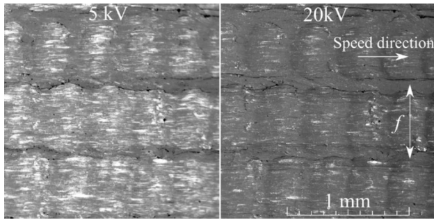
Fig. 21 Surface of machined CuZn38Pb3 captured in backscatter mode at the same location with different acceleration voltages, 5 kV (left) and 20 kV (right). Bright areas show lead
