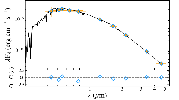
Figure 3. The SED of TOI-1670. Broadband photometry (Table 3) is shown with orange circles, with horizontal errors representing the bandpass width. The best-fitting model SED is shown in black, and the blue diamonds are the model flux integrated over each bandpass. The residuals normalized by the photometric errors are shown in the bottom panel.
