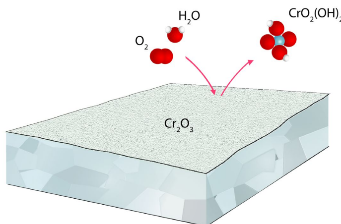
Figure 13 Schematic illustration of chromium evaporation from a chromia scale. Water vapour and oxygen react with the chromia scale, forming CrO 2 (OH) 2 .
