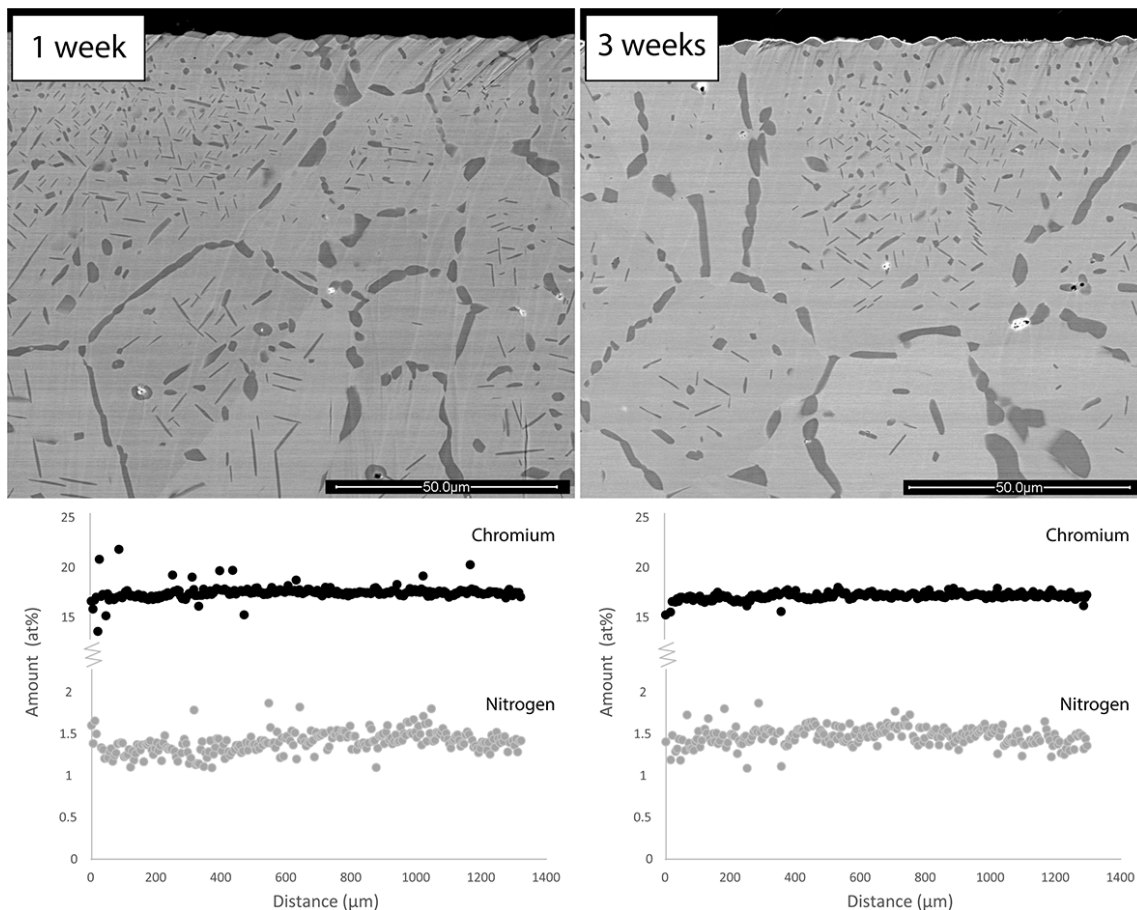
Figure 46 Top: SEM-BSE images of 253 MA after 1 week and 3 weeks of exposure at 1100 °C in a nitriding environment. Bottom: EPMA line-scans in the matrix showing the chromium and nitrogen concentrations through the alloy coupons.
