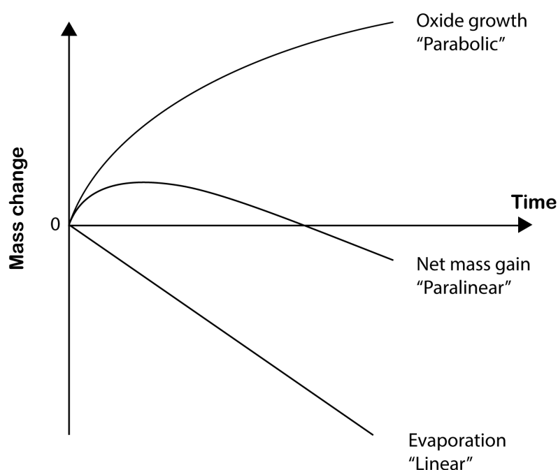
Figure 14 Schematic illustration showing parabolic behaviour of the mass change due to parabolic oxide growth and linear evaporation.
