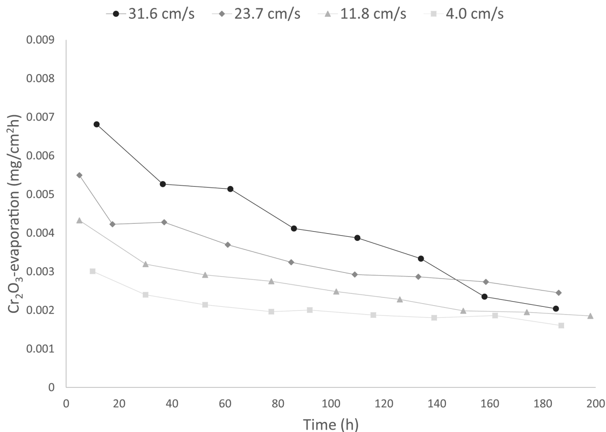
Figure 23 Evaporation rate of \text{Cr}_2\text{O}_3(\text{OH})_2 as a function of exposure time in air + 20% \text{H}_2\text{O} at 800 °C at different gas velocities.
