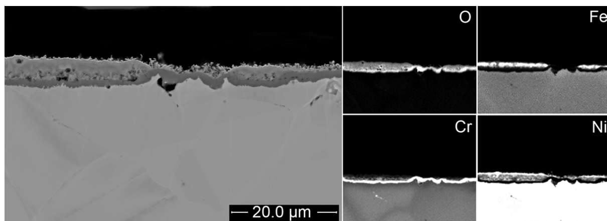
Figure 27 SEM cross-sectional image showing the oxide scale in the bright area after exposure for 200 hours in air + 20% \text{H}_2\text{O} at 800\text{ }^\circ\text{C} and a gas flow velocity of 31.6\text{ cm/s} .
