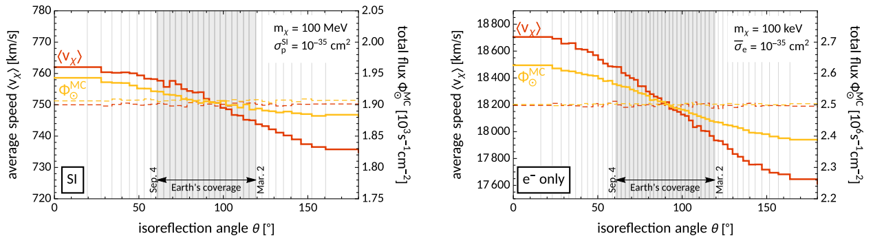
FIG. 12. Anisotropies of the SRDM flux. The figure depicts the total SRDM flux \Phi_{\odot}^{\text{MC}} through Earth (yellow) and the mean speed \langle v_{\chi} \rangle (red) of reflected particles as a function of the isoreflexion angle \theta for SI interactions with nuclei (left) and interactions with electrons only (right). The gray area shows the \theta interval covered by Earth’s elliptical orbit through the Solar System. The dashed lines are the result of MC simulations using isotropic initial conditions, i.e., without the preferred direction of the DM wind, and serve as a consistency check.
