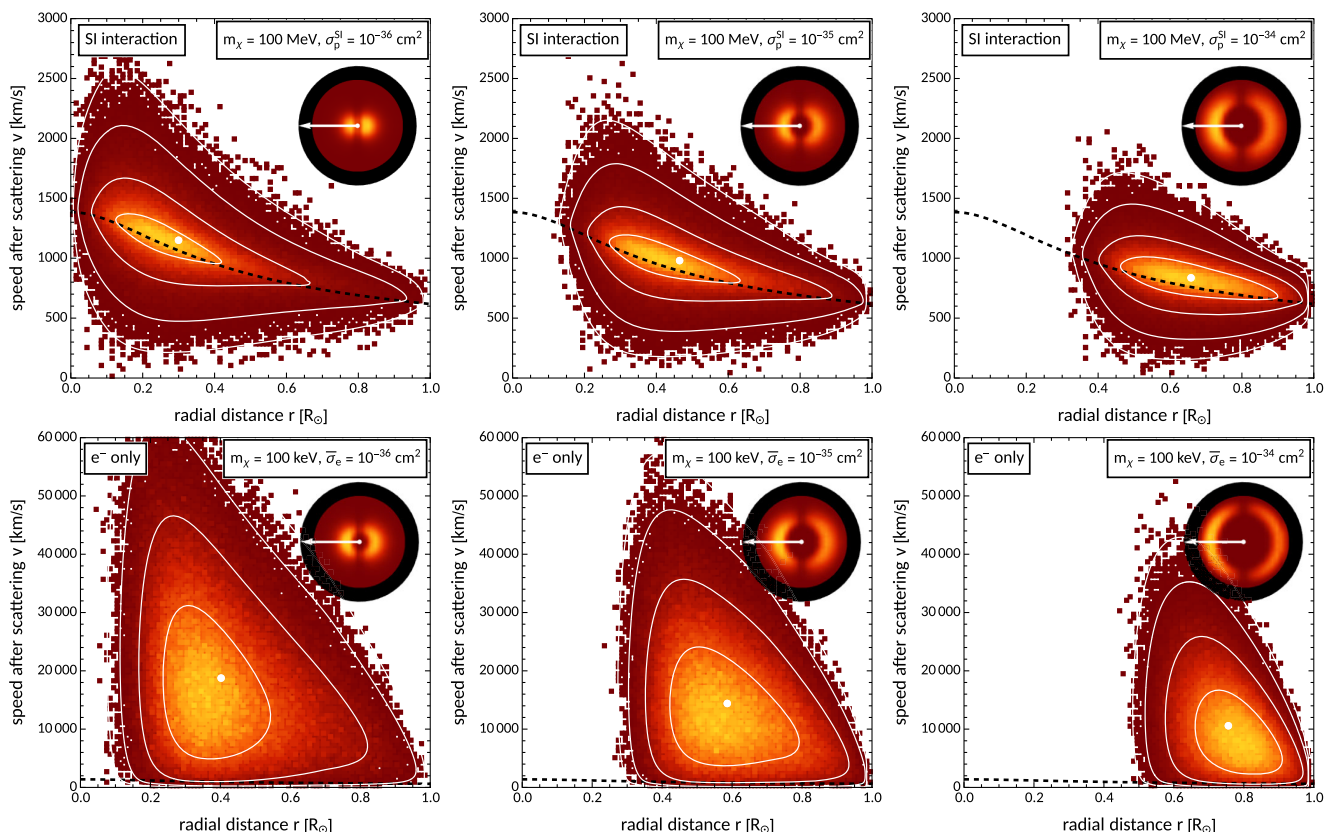
FIG. 8. Two-dimensional histograms of the radial distance r and final DM speed v of the first scattering ( N = 2 \times 10^5 ). The white lines show the analytic differential scattering rate \frac{dS}{dvdr} derived in [50] for comparison. The white dot indicates the maximum, and the contour lines show the differential rate's decline to 50%/10%/1% of the peak's value. The black dashed line gives the local escape velocity; see Eq. (B3) (barely visible in the lower panels). The small inlay figures are an alternative illustration of the distribution of the first scattering's radius, where the white arrow indicates the direction of the Sun's velocity.
