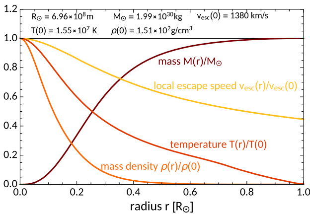
FIG. 18. The standard solar model: The left panel shows the Sun's local escape velocity, mass density, temperature and mass profiles. The right panel depicts the number density of the electrons and nuclei of the solar plasma. The number density of electrons is determined by demanding charge neutrality; see Eq. (B2).
