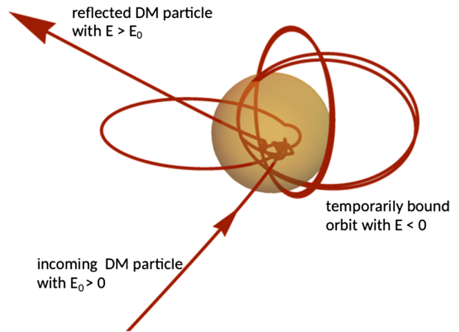
FIG. 1. An illustrative example of a 100 MeV mass DM particle’s trajectory through the Sun obtained with MC simulations. After having scattered around 60 times on solar nuclei, getting decelerated, accelerated, and temporarily captured gravitationally, it finally gets reflected with around 10 times its initial kinetic energy.
