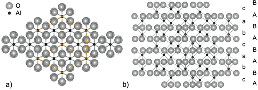
Figure 2.5: The structure of \alpha\text{-Al}_2\text{O}_3 , (a) [0001] projection showing the rhombohedrally centered hexagonal unit cell (b) [11 \bar{2} 0] projection showing the complete stacking sequence of O and Al layers that form ...A-a-B-b-A-c-B-a-A-b-B-c-A..., reproduced from [46]
