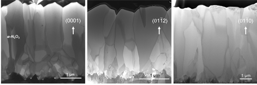
Figure 2.6: Scanning transmission electron microscope (STEM) images showing the microstructure of \alpha - \text{Al}_2\text{O}_3 coatings grown by CVD with \{0001\} , \{01\bar{1}2\} and \{01\bar{1}0\} textures.
