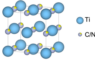
Figure 3.17: FCC rock salt crystal structure of \text{Ti(C,N)} [69]
