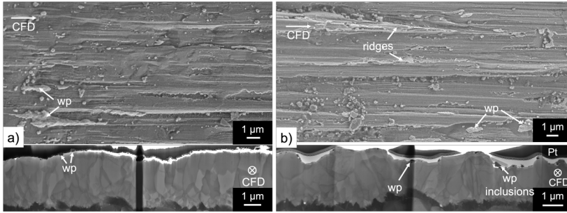
Figure 6.10: SEM secondary electron micrograph of the surface morphology (top) and STEM BF micrograph showing the cross-section (bottom) of the alumina layer in the sliding zone for (a) (0001) texture and (b) (11 \bar{2} 0) texture. Some features in the figures are indicated with arrows. Chip flow direction (CFD) is marked in the figures. Reproduced from Paper IV.
