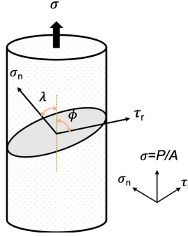
Figure 3.15: Schematic of applied stress on a crystal together with the normal and shear stress components on the slip plane.
