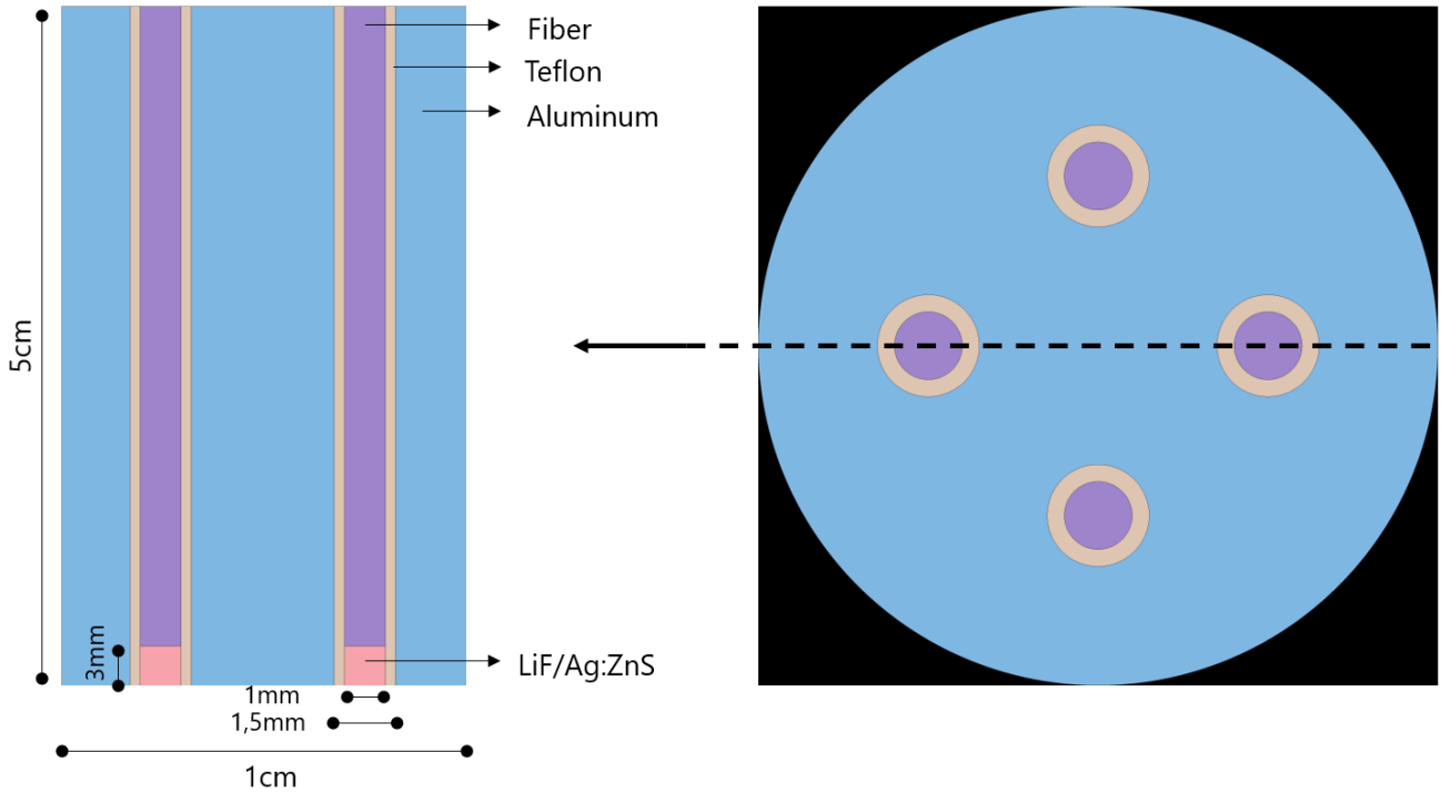
Figure 2.2: LiF-based gradient detector as modelled in Serpent.
