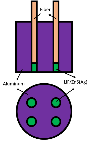
Figure 2.1: Vertical and horizontal cross section view of the detector concept.
