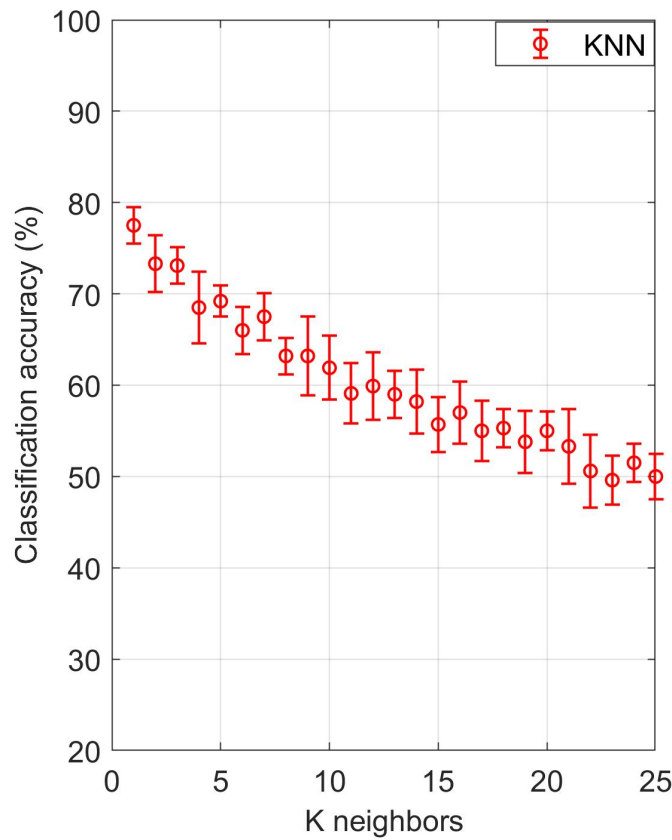
Figure 4.6: Classification accuracy of the kNN algorithm.
