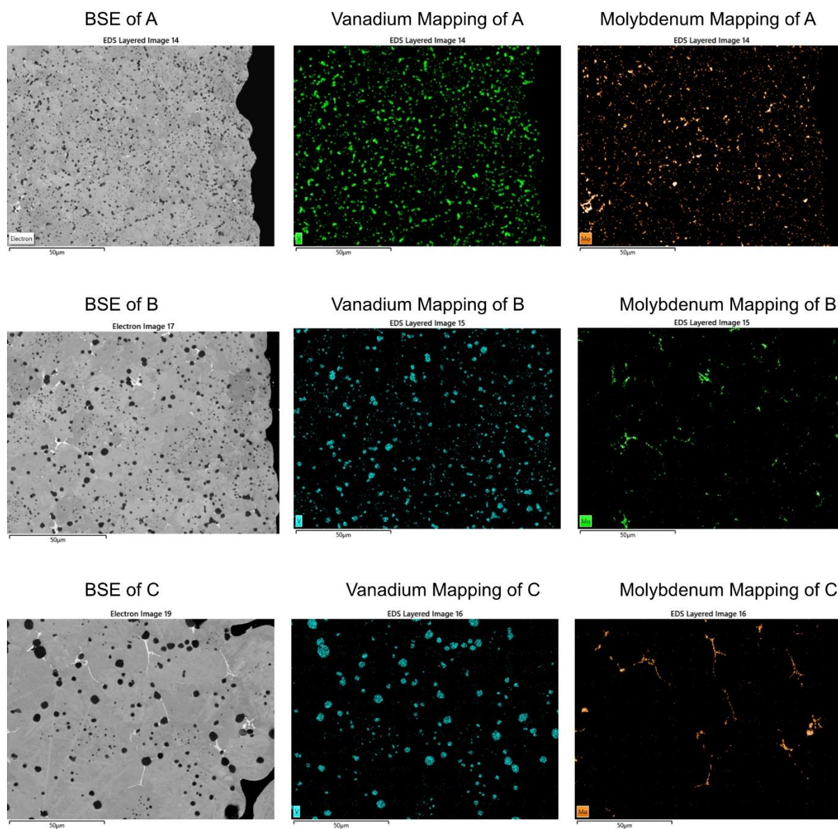
Figure 15. SEM images and EDS mapping of Vanadis 4E material after sintering at (a) 1150 °C, sample A, (b) 1200 °C, sample B and (c) 1250 °C, sample C and followed by capsule-free HIP
