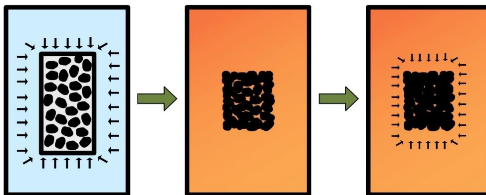
Figure 5. Schematics of procedure to obtain high density via cold isostatic pressing (CIP), sintering and capsule-free hot isostatic pressing (capsule-free HIP).
