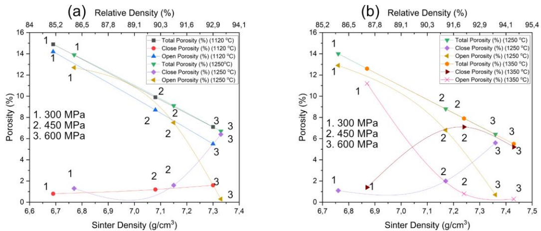
Figure 6. Plot of measured open and closed porosities as function of sintered density for sintering in (a) 90N 2 /10H 2 and (b) vacuum (10 -2 mbar)
