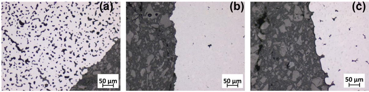
Figure 13. Pore morphology of Vanadis 4E material after sintering at (a) 1150 °C, (b) 1200 °C and (c) 1250 °C
