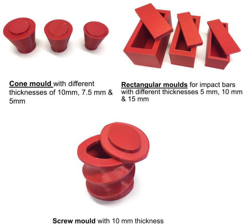
Figure 2. The 3D printed moulds made from thermoplastic polyurethane filaments using ZYXX+ FDM printer.
