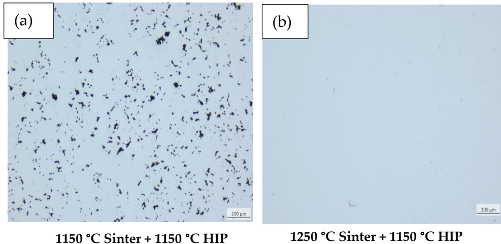
Figure 9. light optical microscopy images of CrA-2Ni-0.3C samples after (a) 1150 °C sintering in HIP furnace + 1150 °C capsule-free HIP (a) 1250 °C sintering in HIP furnace + 1150 °C capsule-free HIP.
