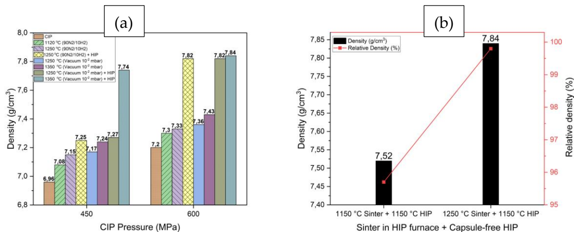
Figure 8. Density measurements of CrA-2Ni-0.3C after (a) CIP+Sinter+Capsule-free HIP (b) CIP+Sinter in HIP+Capsule-free HIP
