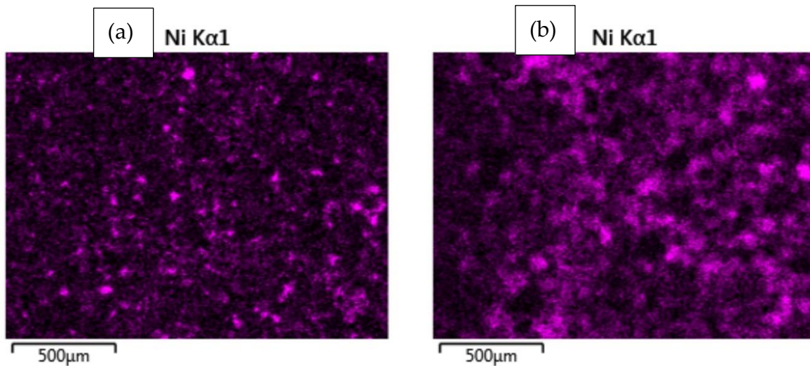
Figure 10. EDS Mapping for nickel in CrA-2Ni-0.3C after sintering at (a) 1120 °C and (b) 1250 °C
