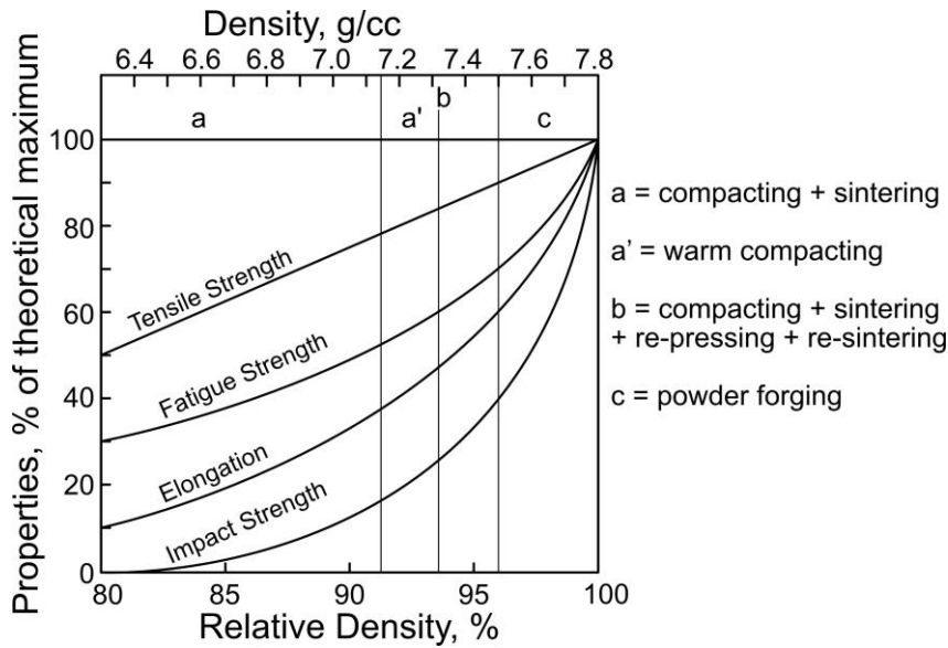
Figure 1. Effect of relative density on the mechanical performance of PM component (redrawn from [50])
