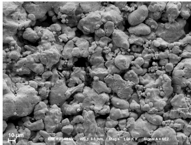
Figure 4. Overview of Cr-alloyed steel powder diffusion-bonded with 2wt%Ni and admixed with 0.3wt%C.
