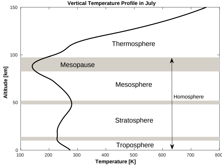
Figure 1.1: Divisions of the atmosphere based on vertical temperature gradient. The vertical temperature profile is obtained from MSISE90 model (Hedin (1991)) in July at the latitude of 80 °N
