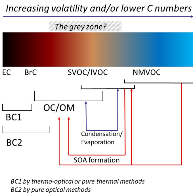
Figure 11. Synoptic description of the carbonaceous species from graphitic carbon (EC) to NMVOCs.
