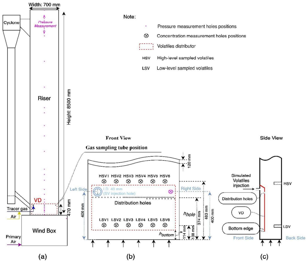
Figure 7. (a) Cold-flow circulating fluidized-bed model equipped with the VD and pressure and \text{CO}_2 concentration measurement systems; (b) Front view of the riser bottom, the distribution holes are seen in detail in Figure 8; (c) Side view, the side view with more details is shown in Figure 10.
