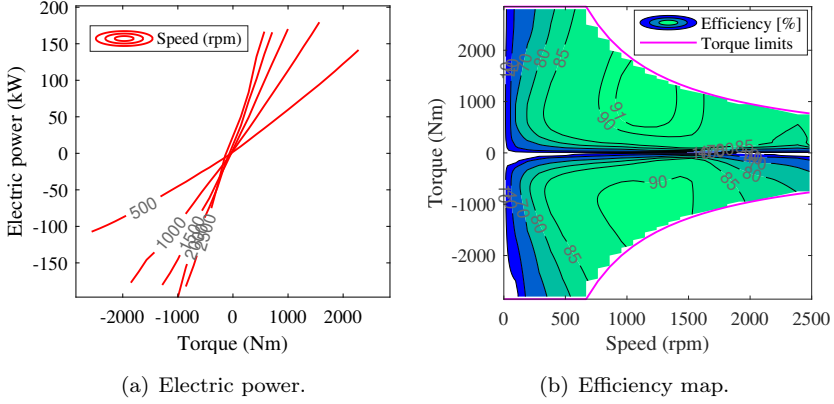
Fig. 6.2: Electric power and efficiency map of the electric machine with the associated inverter. The electric machine torque is limited by speed dependent bounds.
