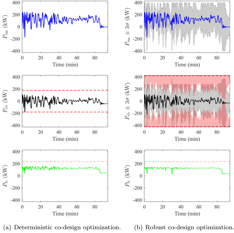
Fig. 7.4: Optimal power distributions.
