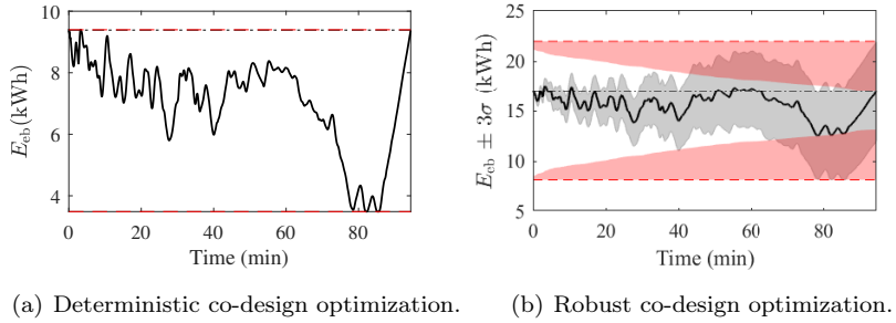
Fig. 7.5: Battery energy trajectories.
