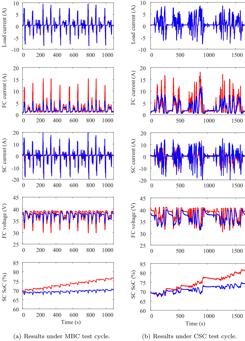
Fig. 5.10: Experimental results for adaptive power split strategy validation with Nexa FC system connected. The load current is applied to the source/sink with a sampling time of 1 s. The red line represents the results under the constant cut-off frequency and the blue line represents the results under the adaptive cut-off frequency.
