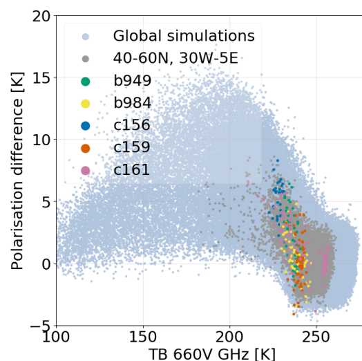
Figure 5. The scatter plot showing the PD vs. TB_V at 660 GHz. The light blue dots are near-global simulations; the grey dots denote simulations in 40^\circ\text{N} – 60^\circ\text{N}/30^\circ\text{W} – 5^\circ\text{E} . The five alphanumeric codes depict observations from the five flight campaigns described by Fox [61].
